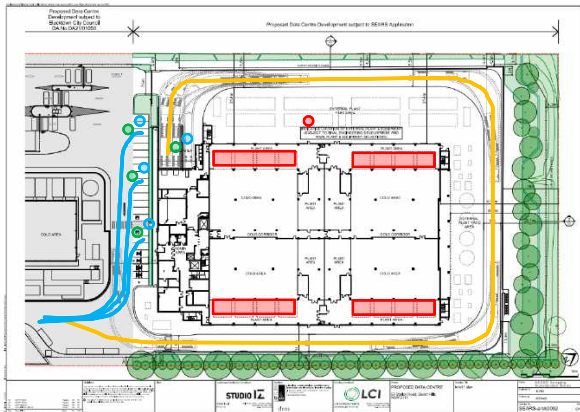
Figure 11 Modelled Noise Emission Sources visualized for the Day/Evening Period
