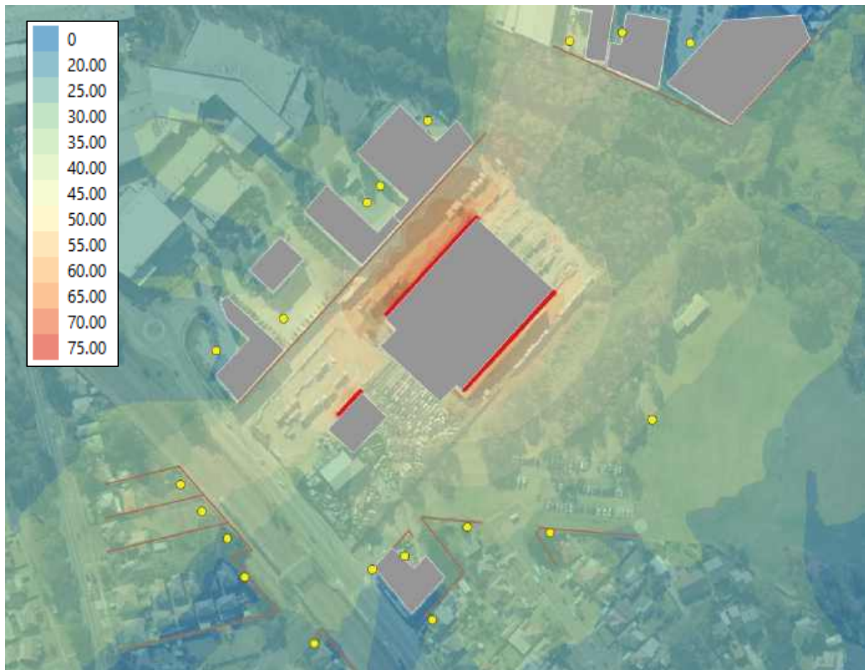
Figure 14 Standard Mode Operational Scenario 2 – Operational Evening/Night Scenario with 60 Direct Evaporative Cooling Air Handling Units (with 200mm Deep Acoustic Louvres)
