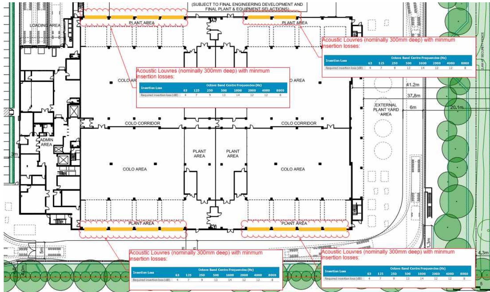
Figure 19 Markup showing locations of proposed acoustic louvres should "Bushfire mode" AHUs be implemented – Level 1
