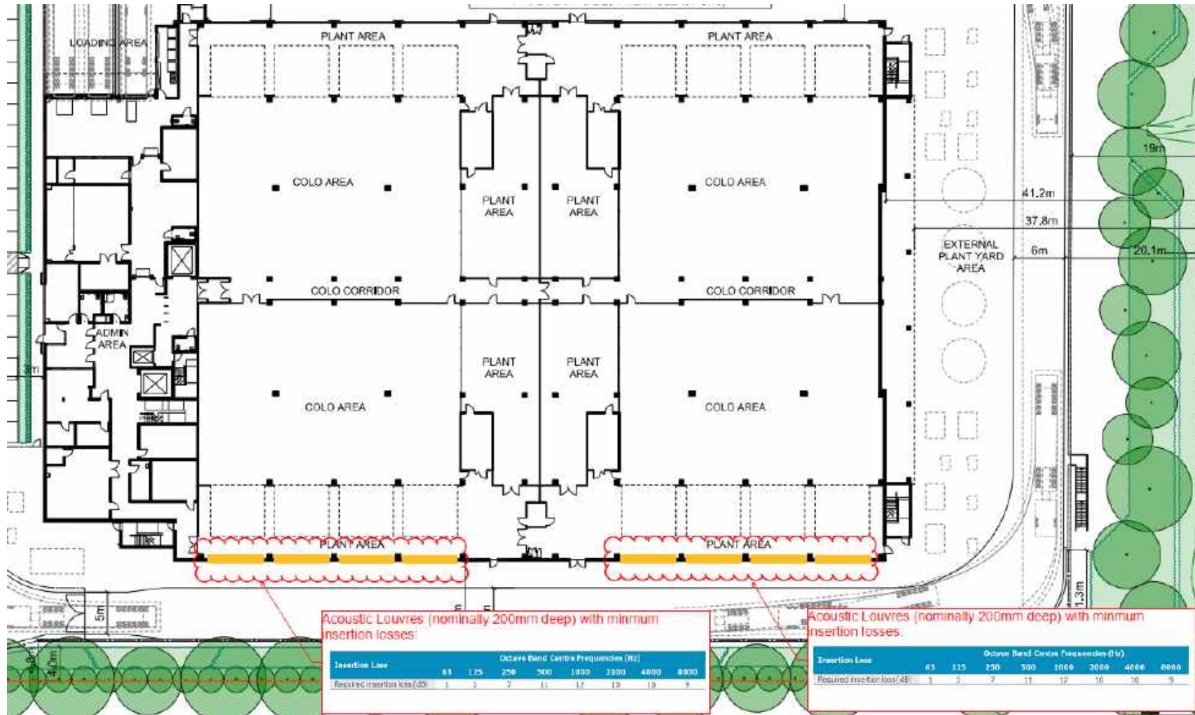
Figure 17 Markup showing locations of proposed acoustic louvres should "Standard mode" AHUs be implemented – Level 1
