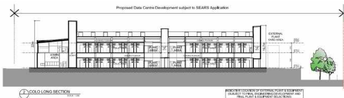
Figure 5 Section View of Proposed SYD08 Development
