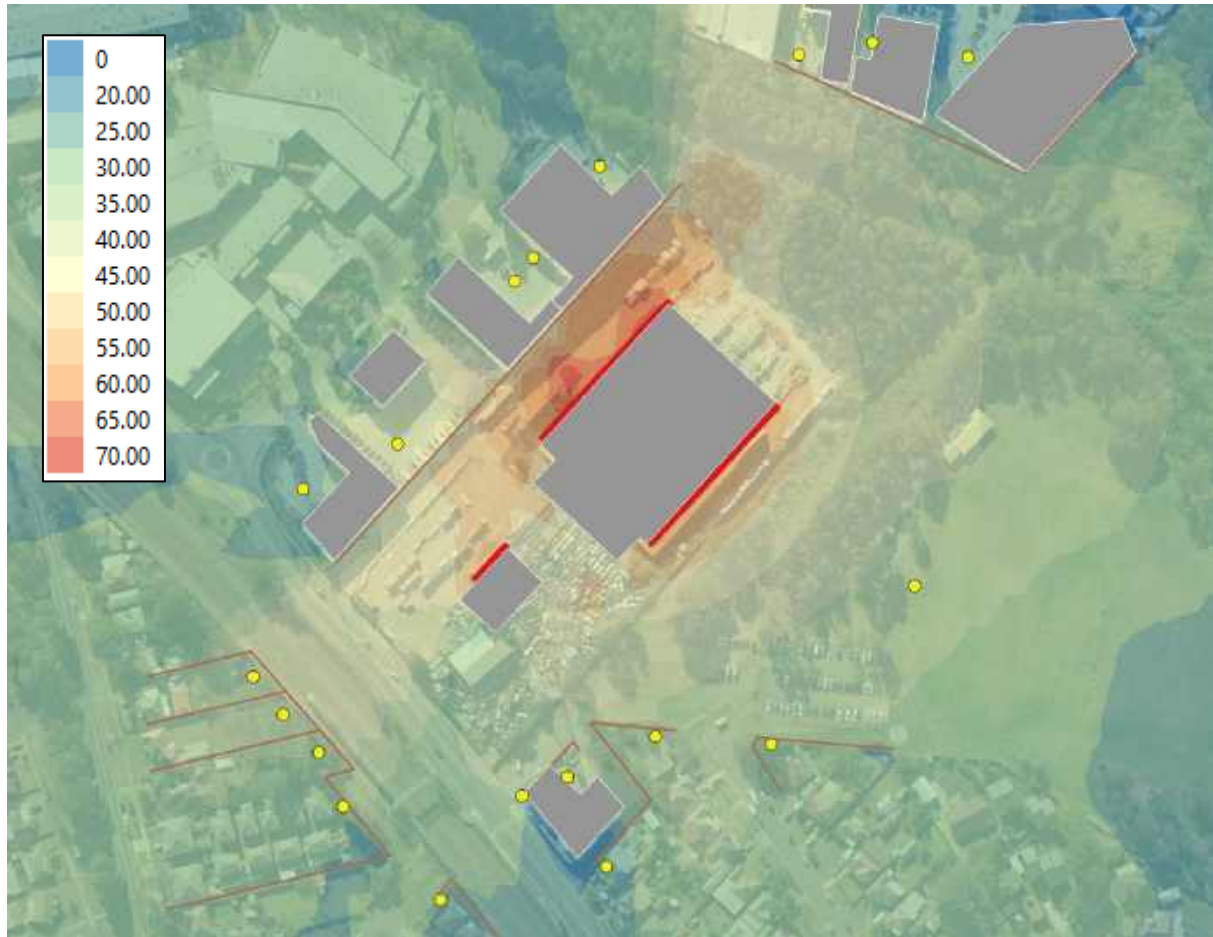
Figure 15 Bushfire Mode Operational Scenario 1 – Operational Day Scenario with 67 Direct Evaporative Cooling Air Handling Units (with 300mm Deep Acoustic Louvres) and 1 x 3.0 MW Generator
