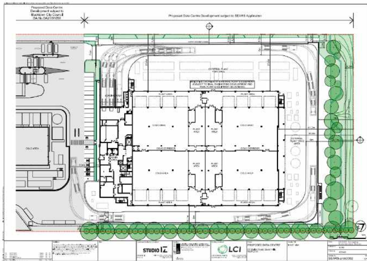
Figure 4 Proposed SYD08 Site Plan
