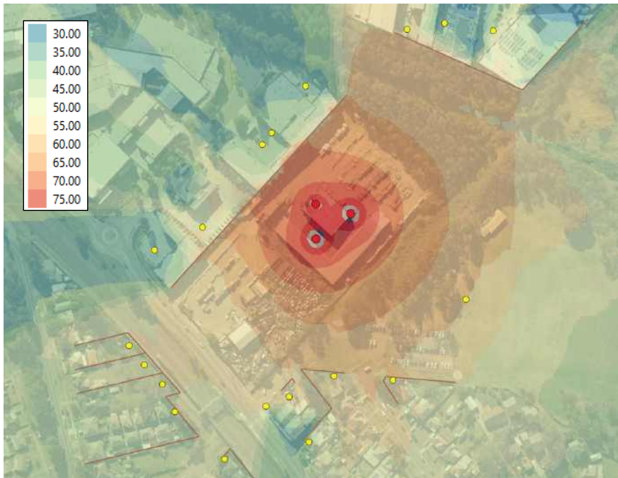
Figure 25 Predicted Noise Contours – Construction Scenario 2, L_{Aeq} (15 minute)
