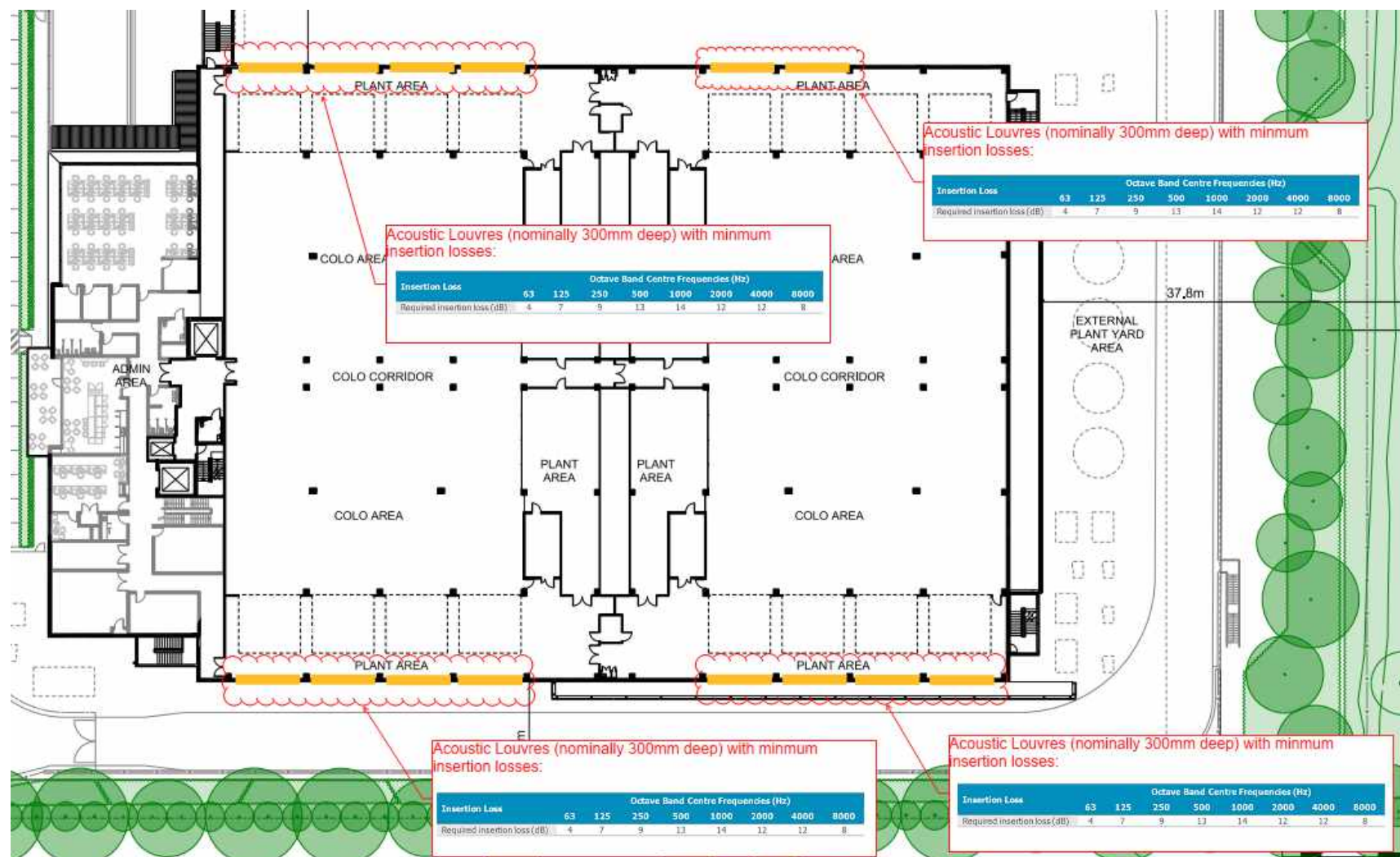
Figure 20 Markup showing locations of proposed acoustic louvres should "Bushfire mode" AHUs be implemented – Level 2
