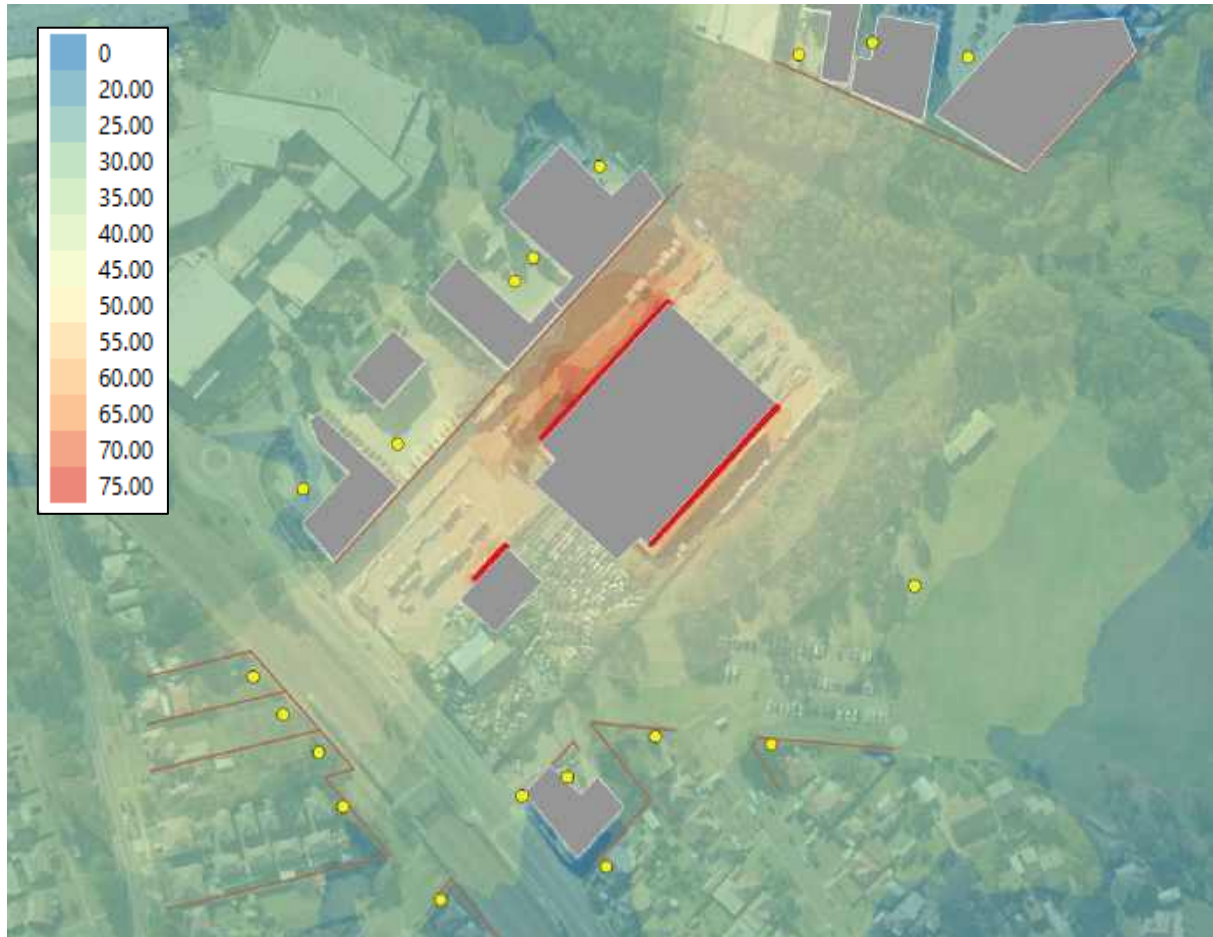
Figure 13 Standard Mode Operational Scenario 1 – Operational Day Scenario with 60 Direct Evaporative Cooling Air Handling Units (with 200mm Deep Acoustic Louvres) and 1 x 3.0 MW Generator
