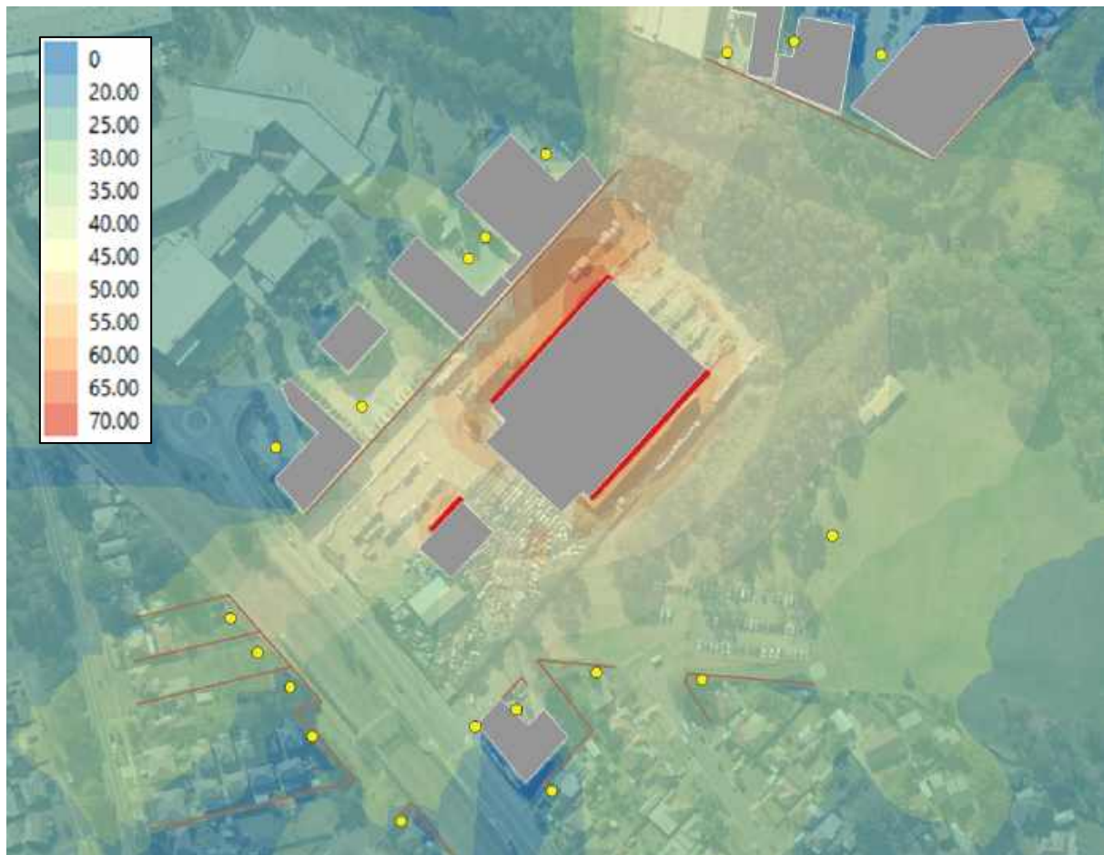
Figure 16 Bushfire Mode Operational Scenario 2 – Operational Evening/Night Scenario with 67 Direct Evaporative Cooling Air Handling Units (with 300mm Deep Acoustic Louvres)
