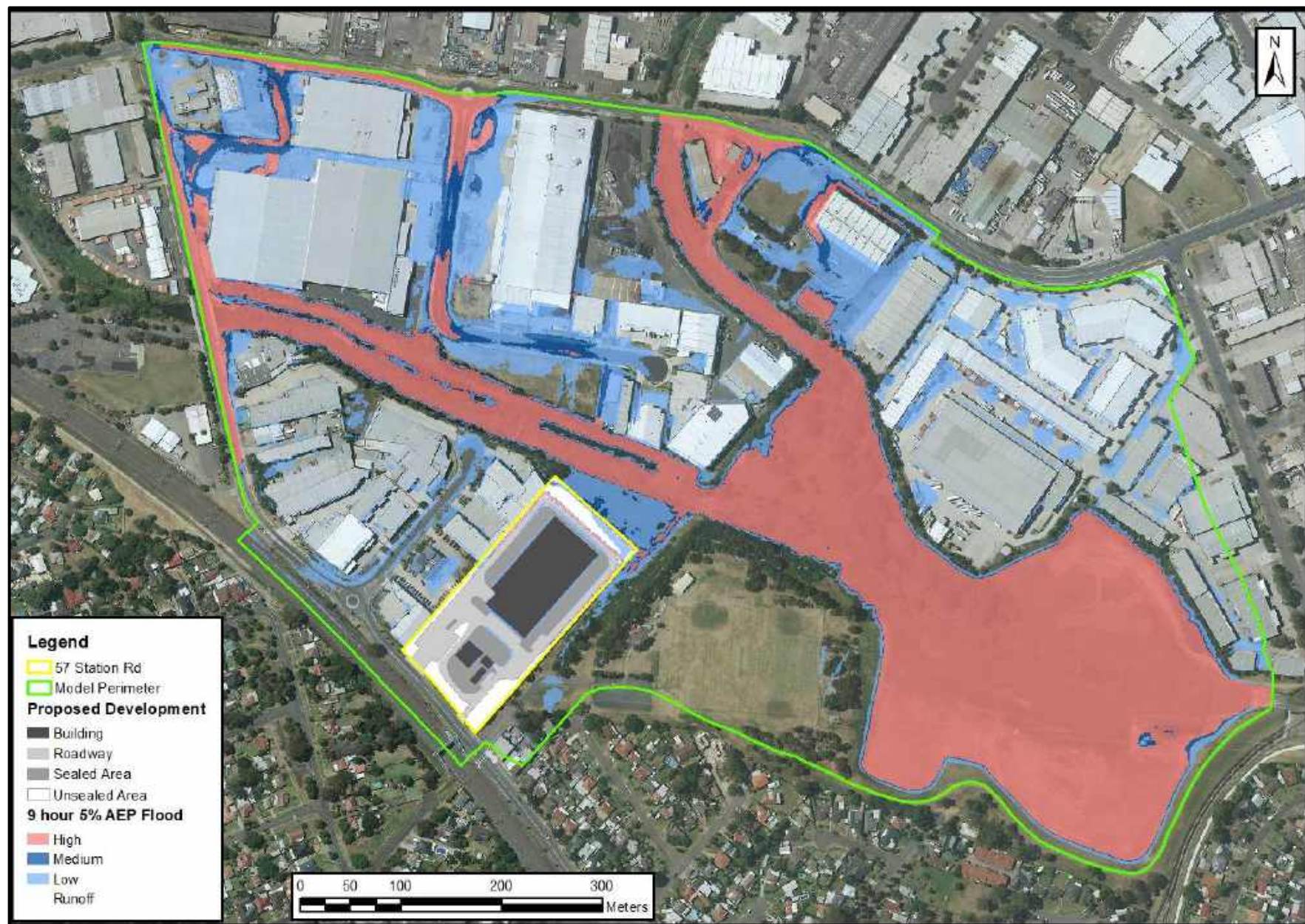
Figure F7: Design 9 hour 5% AEP Flood Extent
