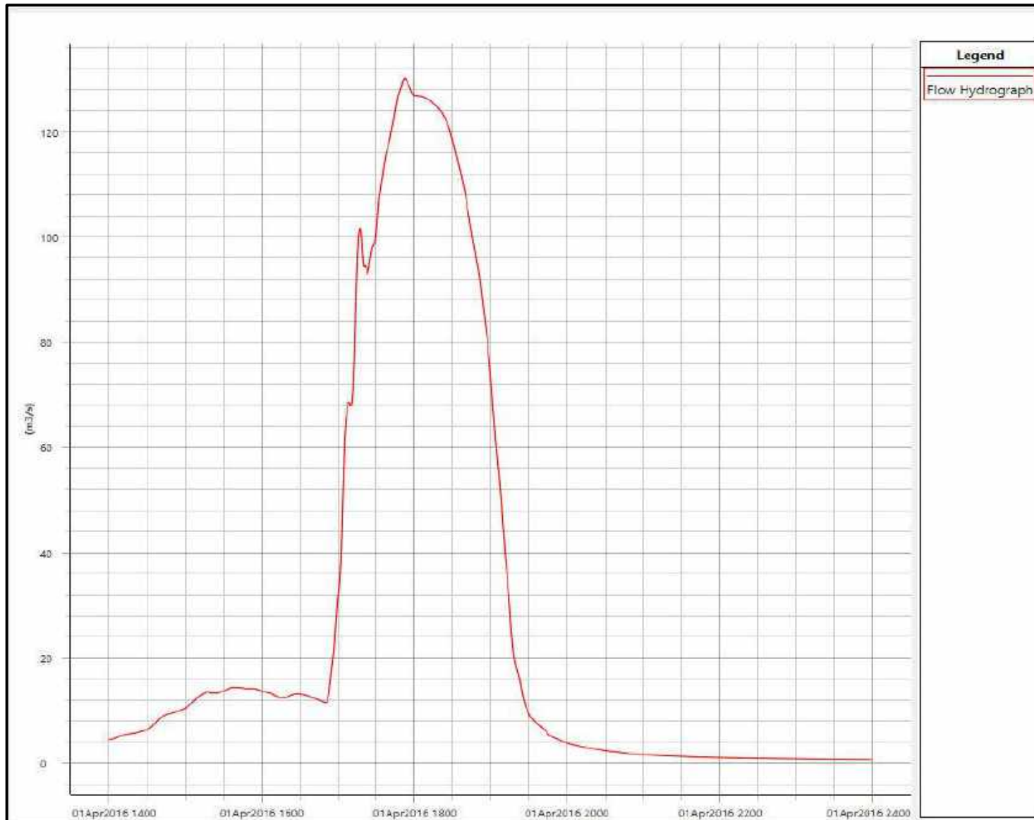
Figure E24 : Inflow Hydrograph at Boundary TGC01.24T
