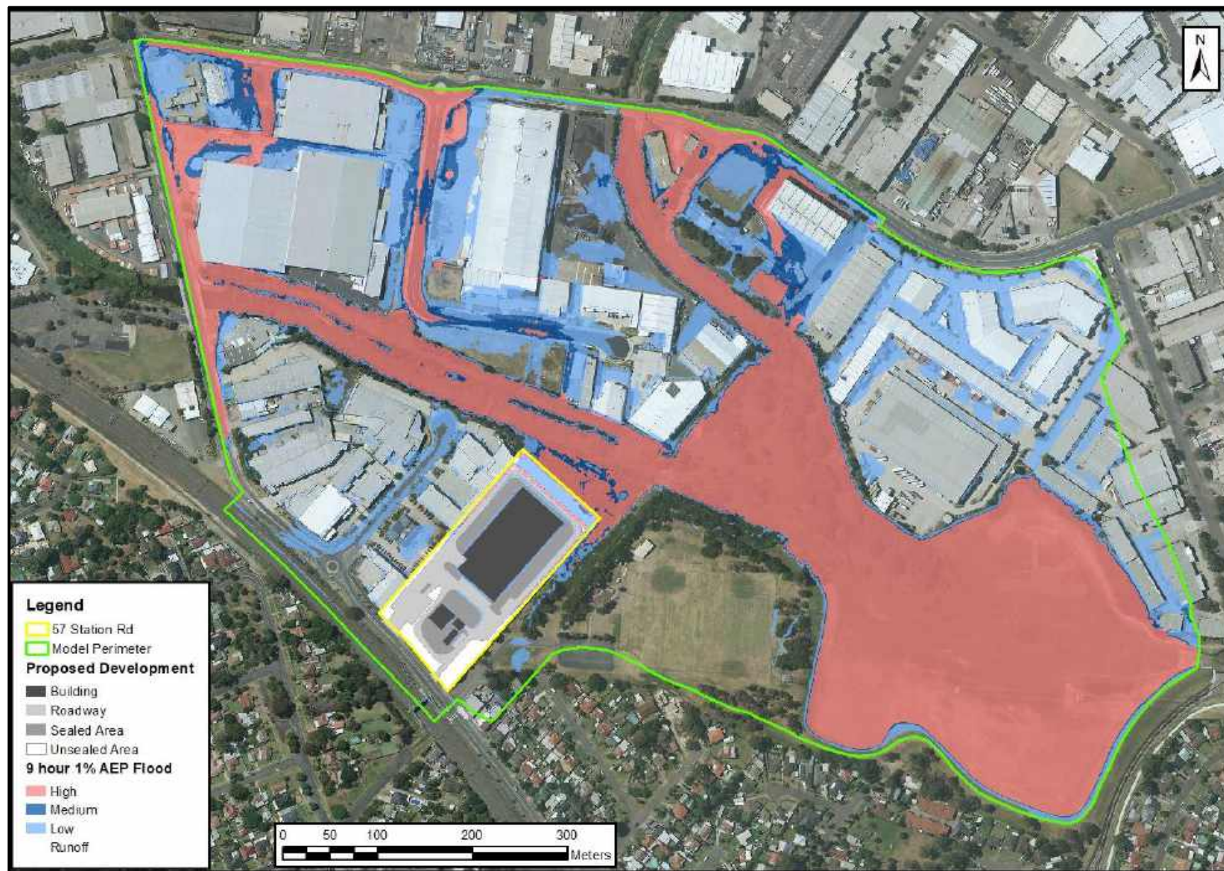
Figure F6: Design 9 hour 1% AEP Flood Extent
