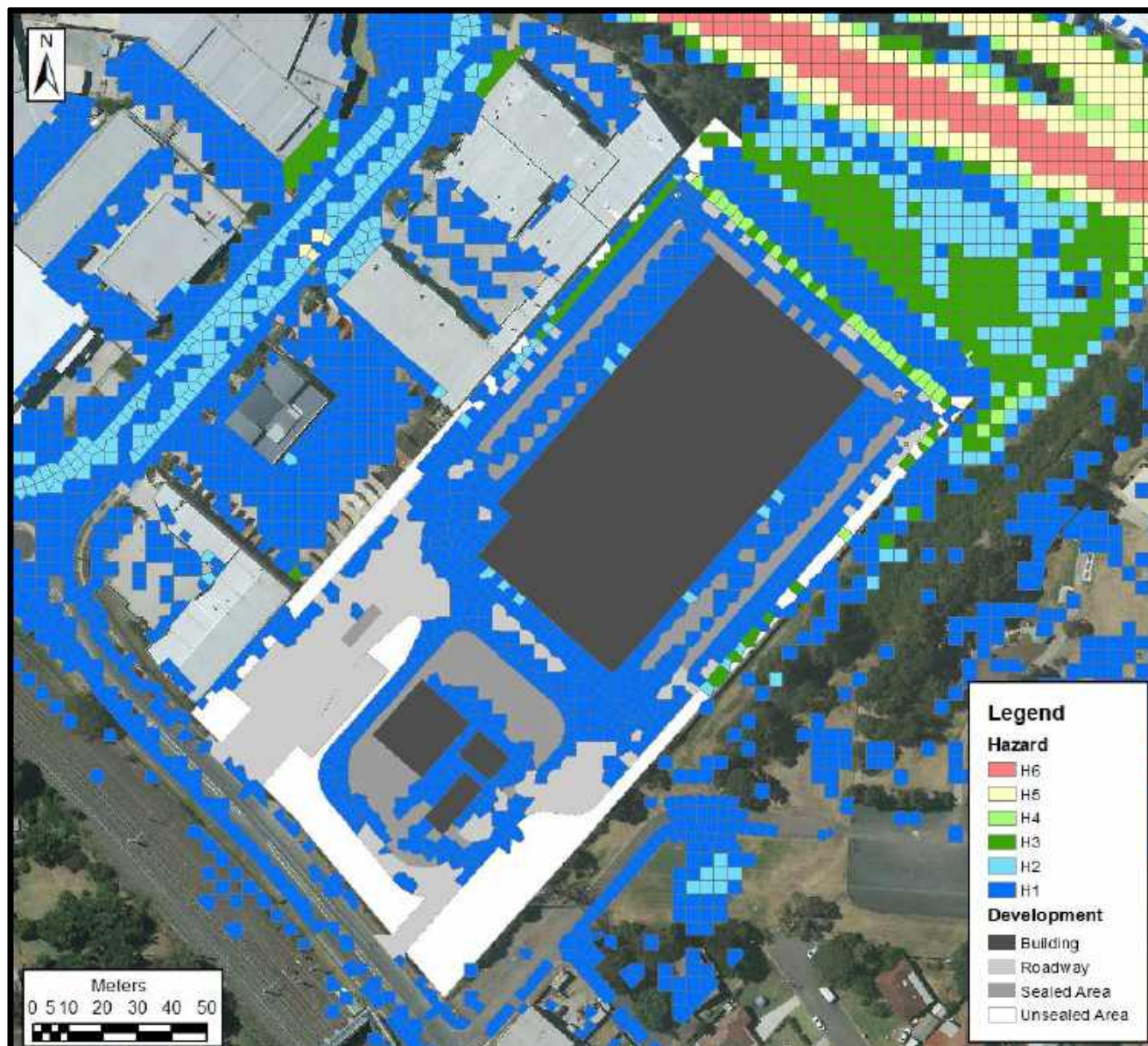
Figure G9: Design 25 min 1% AEP Hydraulic Hazard for the Site.
