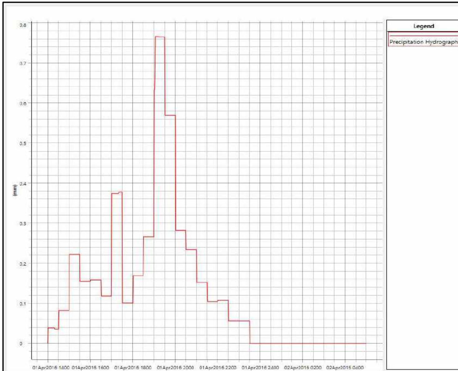
Figure E20 : Precipitation Excess for Flow Area StationRd_FA
