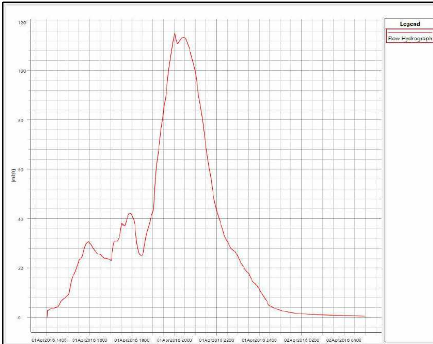
Figure E19 : Inflow Hydrograph at Boundary TGC01.24T
