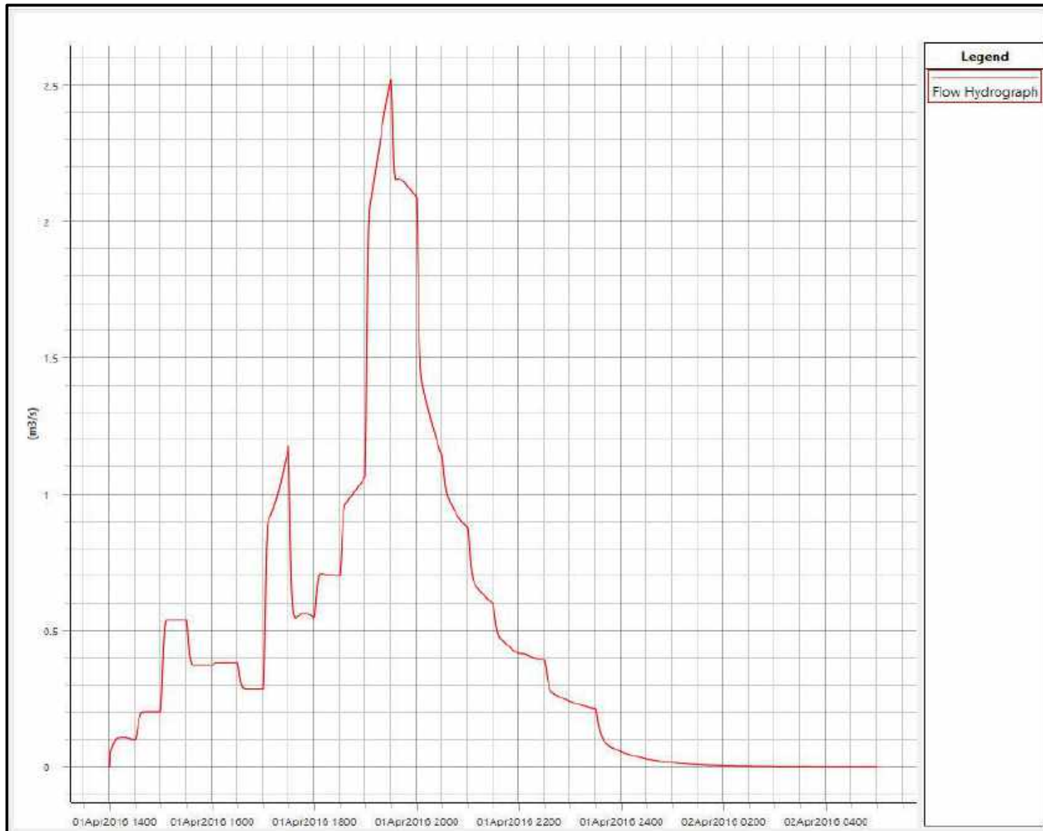
Figure E13 : Inflow Hydrograph at Boundary BTN31.00T
