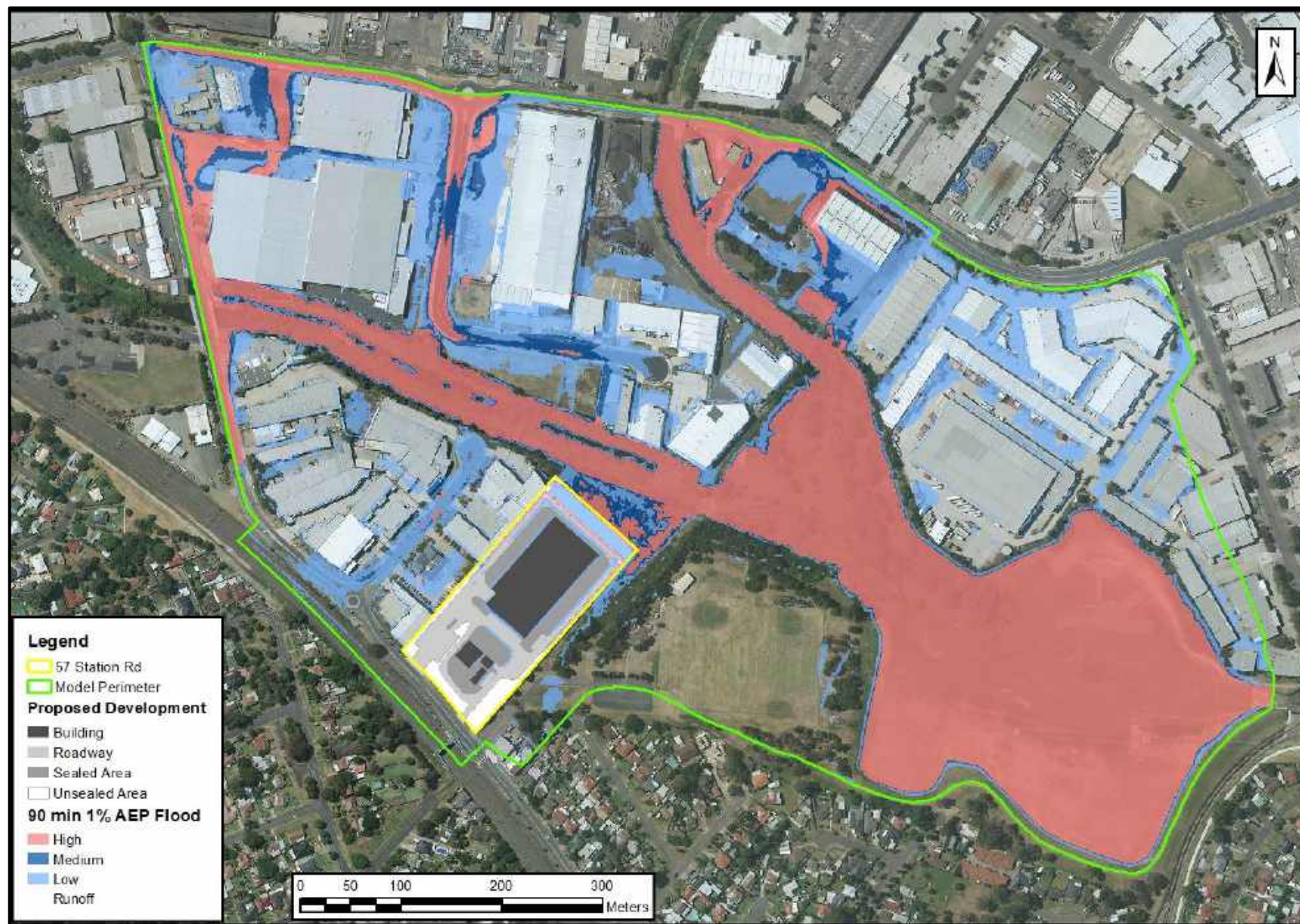
Figure F8: Design 90 min 1% AEP Flood Extent
