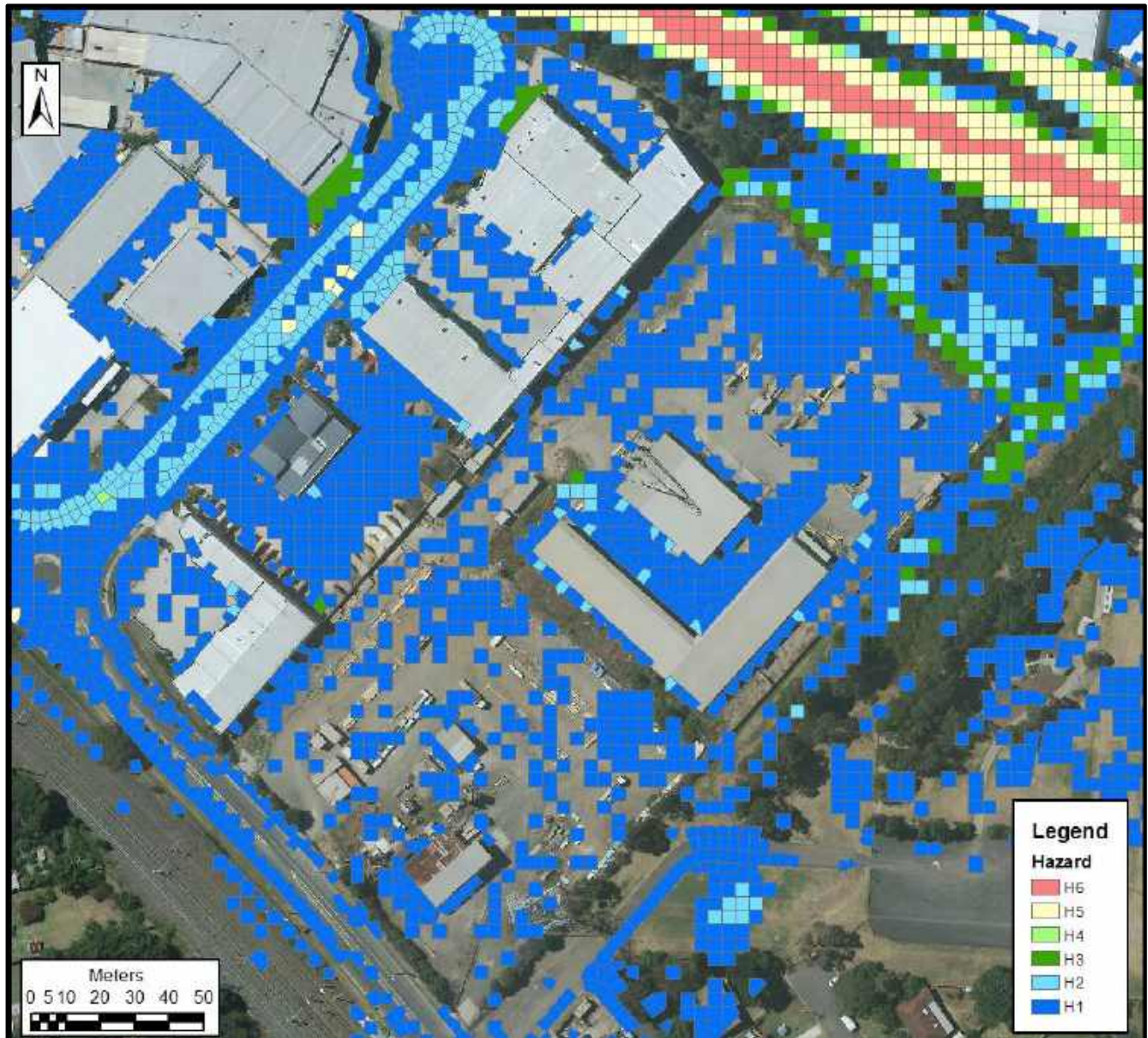
Figure G5: Existing 15 min 1% AEP Hydraulic Hazard for the Site.
