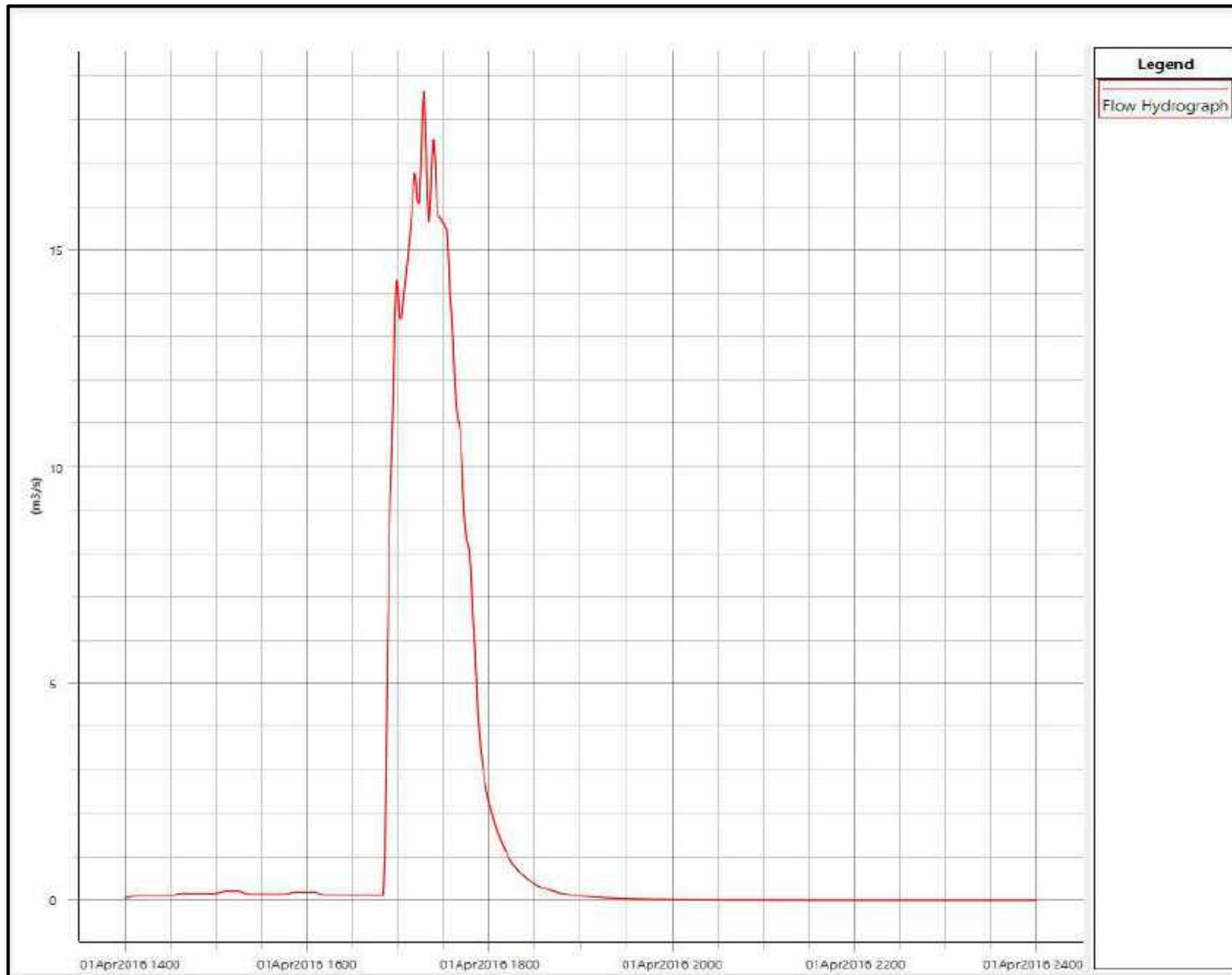
Figure E23 : Inflow Hydrograph at Boundary BTN31.00T
