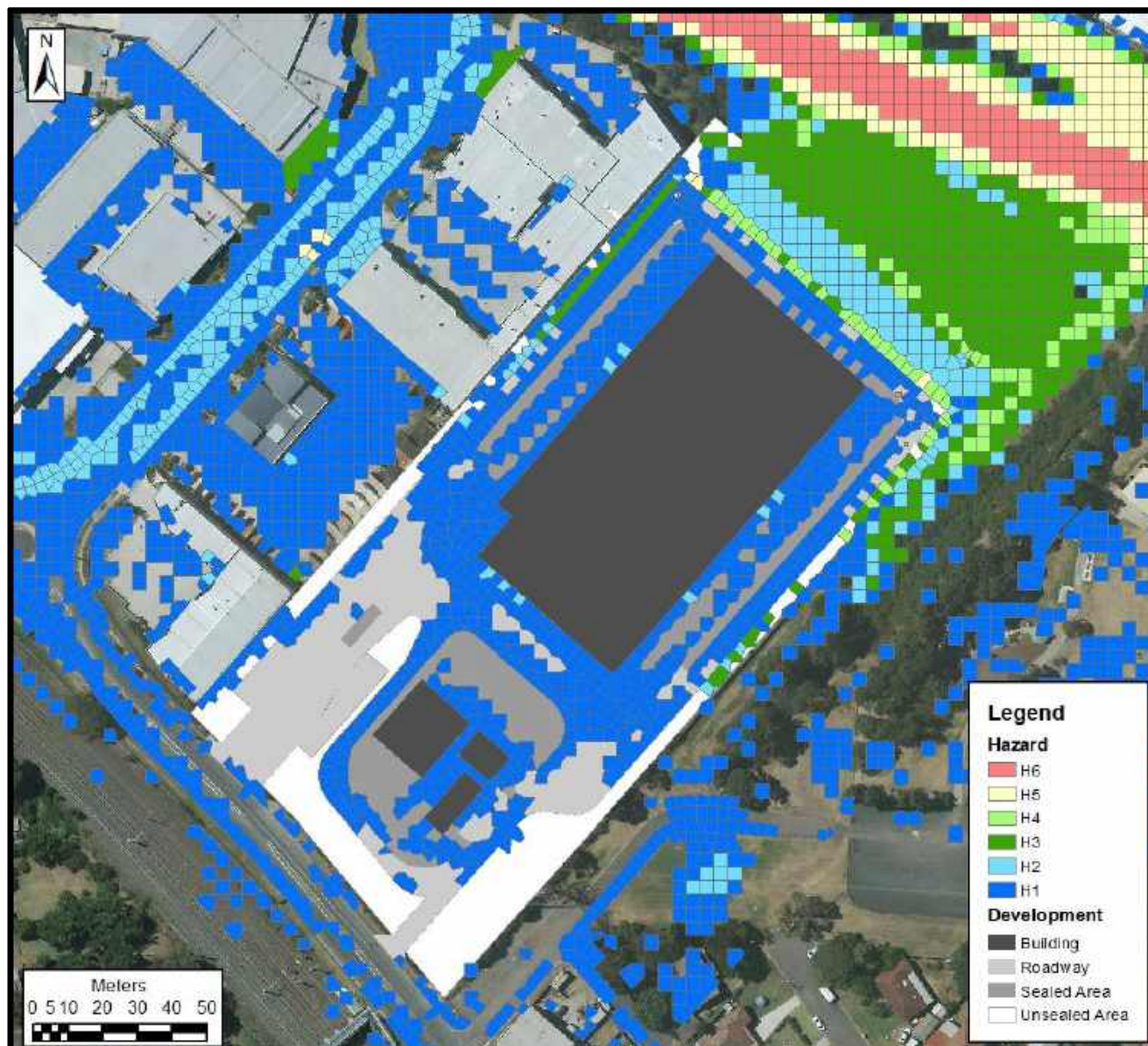
Figure G8: Design 90 min 1% AEP Hydraulic Hazard for the Site.
