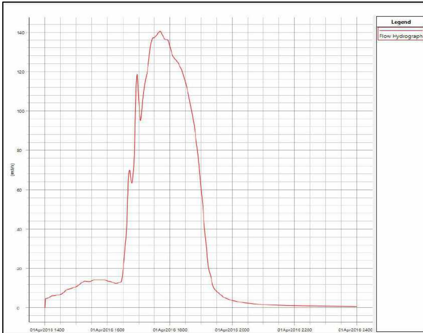
Figure E29 : Inflow Hydrograph at Boundary TGC01.24T
