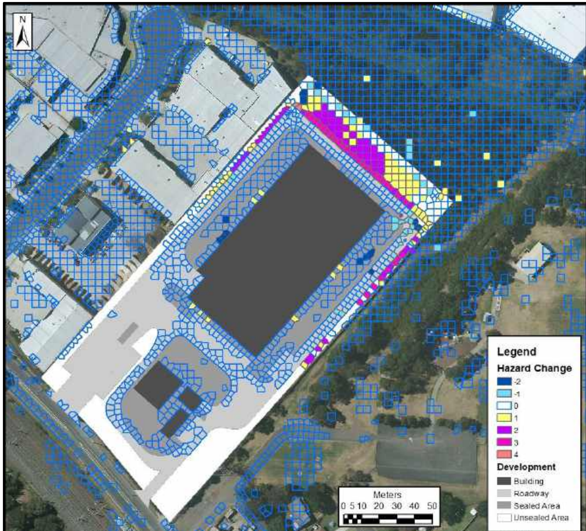
Figure 15 : 9 hour 1% AEP Flood Event Hydraulic Hazard Comparison, Design Scenario to Existing Scenario
