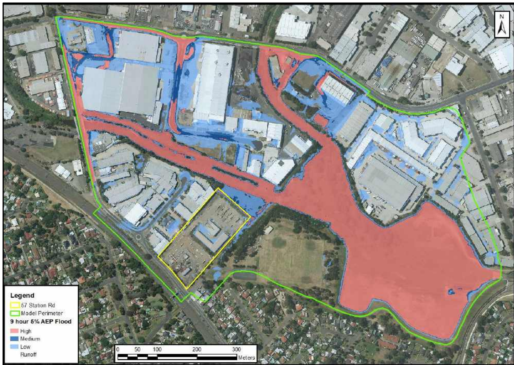
Figure F2: Existing 9 hour 5% AEP Flood Extent
