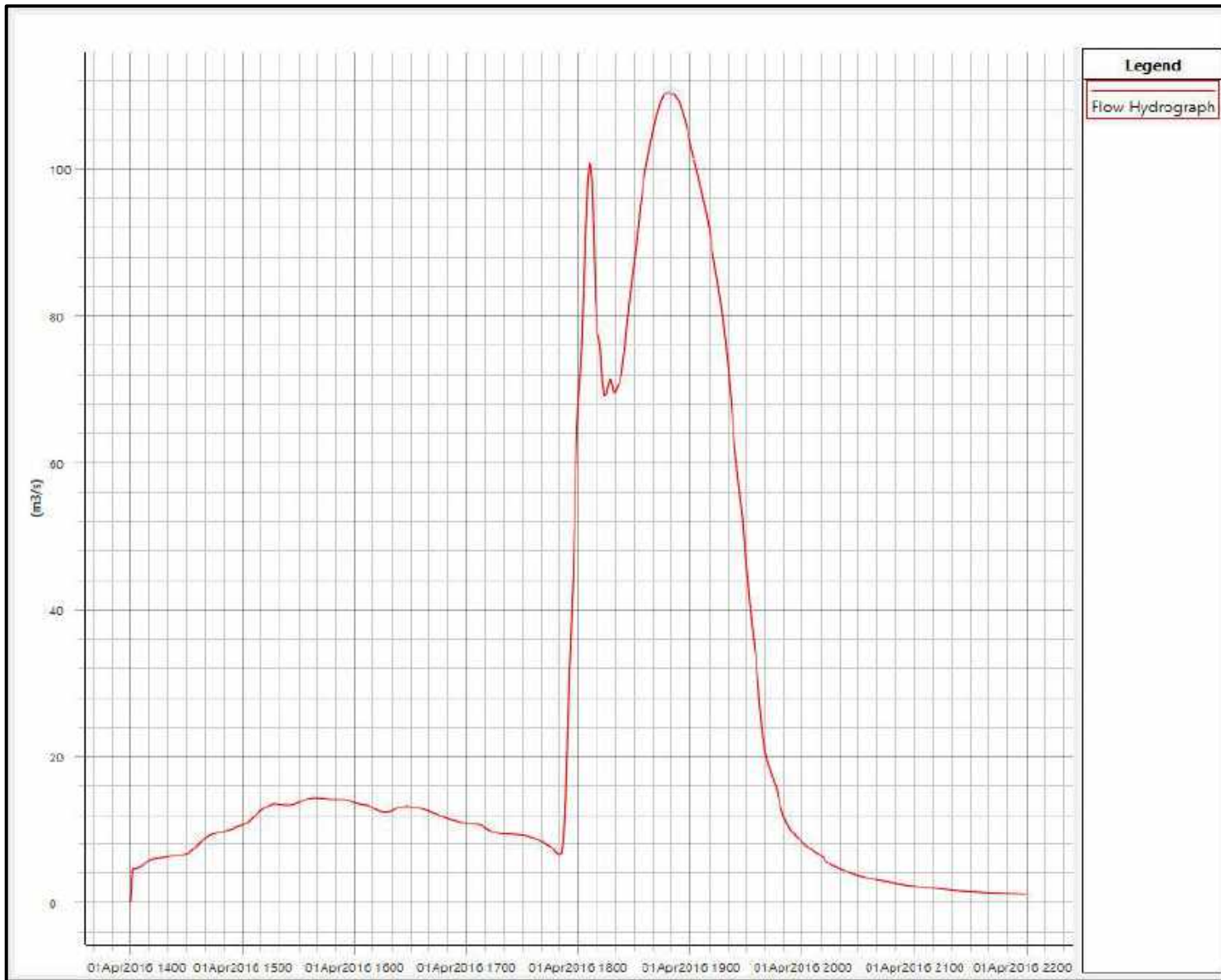
Figure E34 : Inflow Hydrograph at Boundary TGC01.24T
