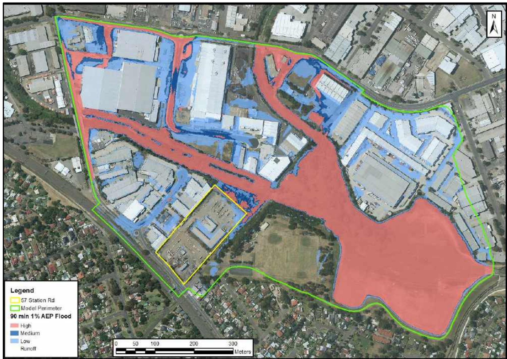
Figure F3: Existing 90 min 1% AEP Flood Extent
