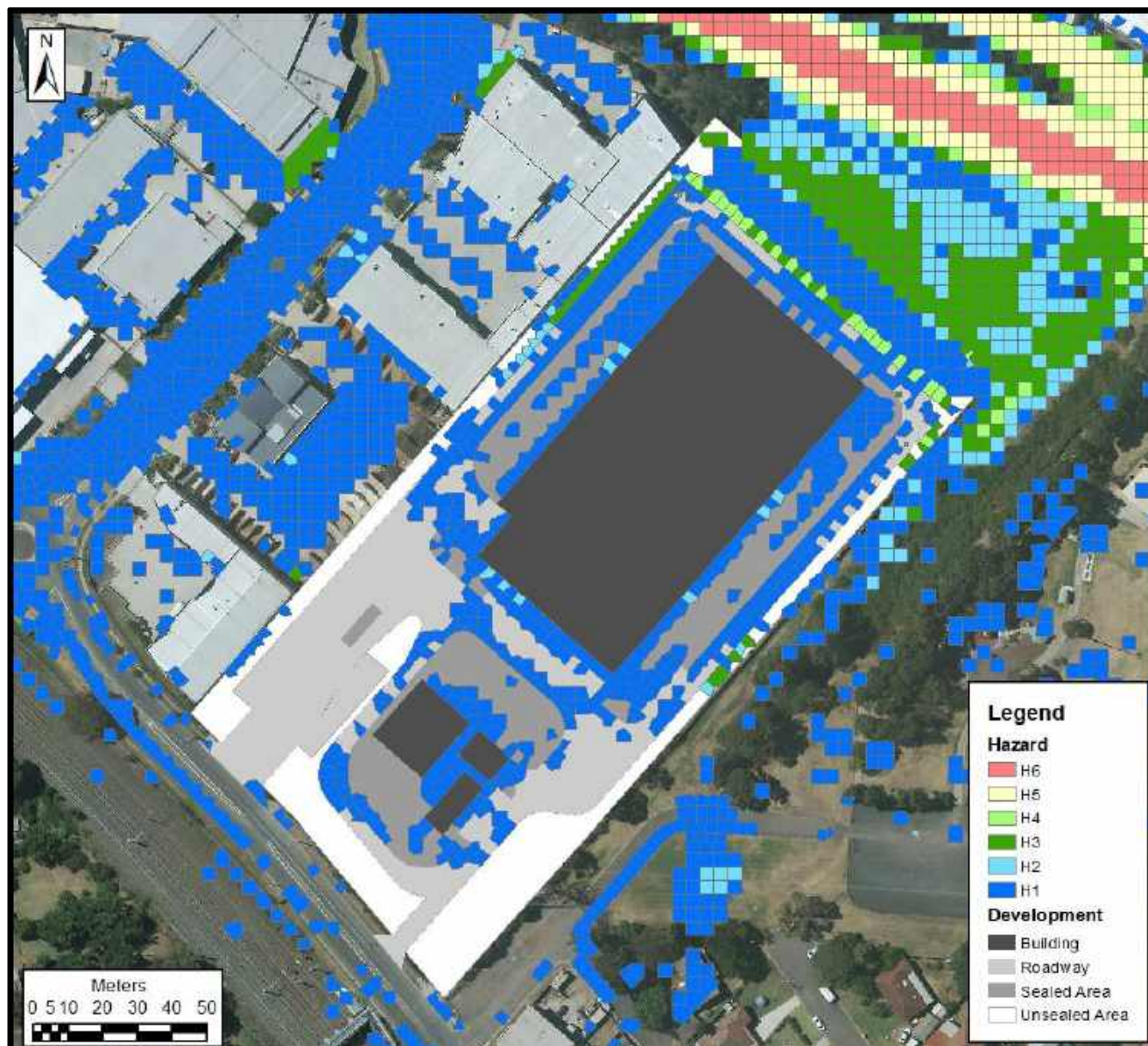
Figure G7: Design 9 hour 5% AEP Hydraulic Hazard for the Site.
