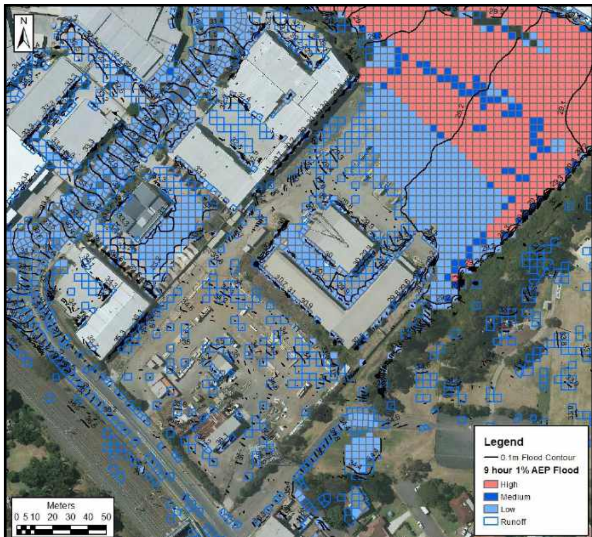
Figure 7: 1% AEP Flood Inundation Extent in vicinity of the site, Existing Scenario (Calibrated Model)
