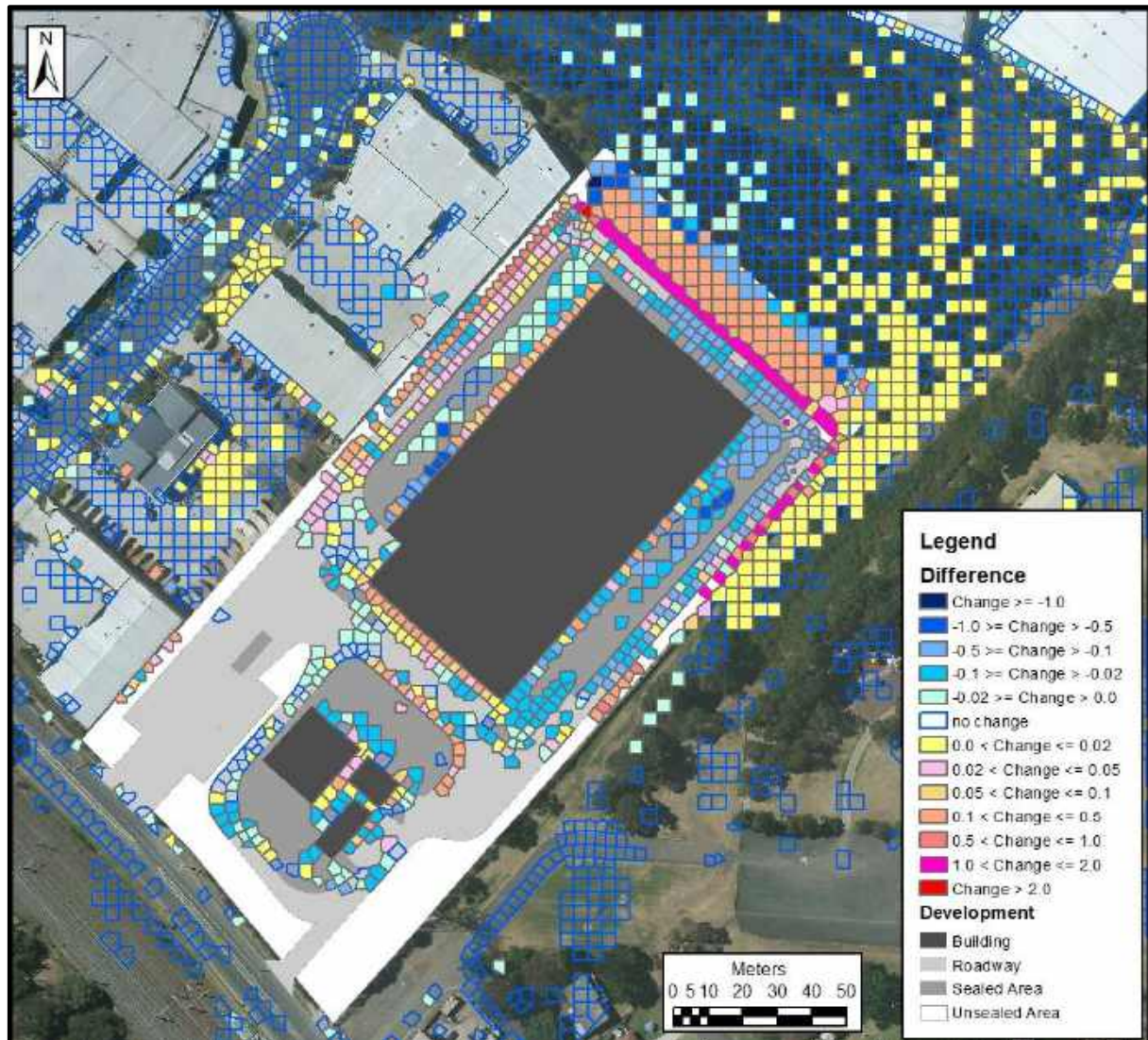
Figure 14 : 1% AEP Flood Inundation Depth Comparison, Design Scenario to Existing Scenario
