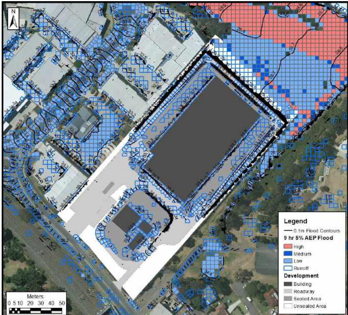
Figure 13 : 5% AEP Flood Inundation Extent, Design Scenario
