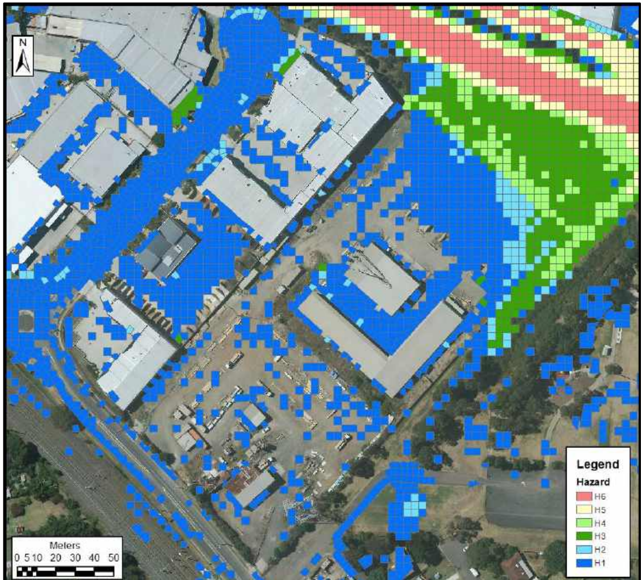
Figure G1: Existing 9 hour 1% AEP Hydraulic Hazard for the Site.
