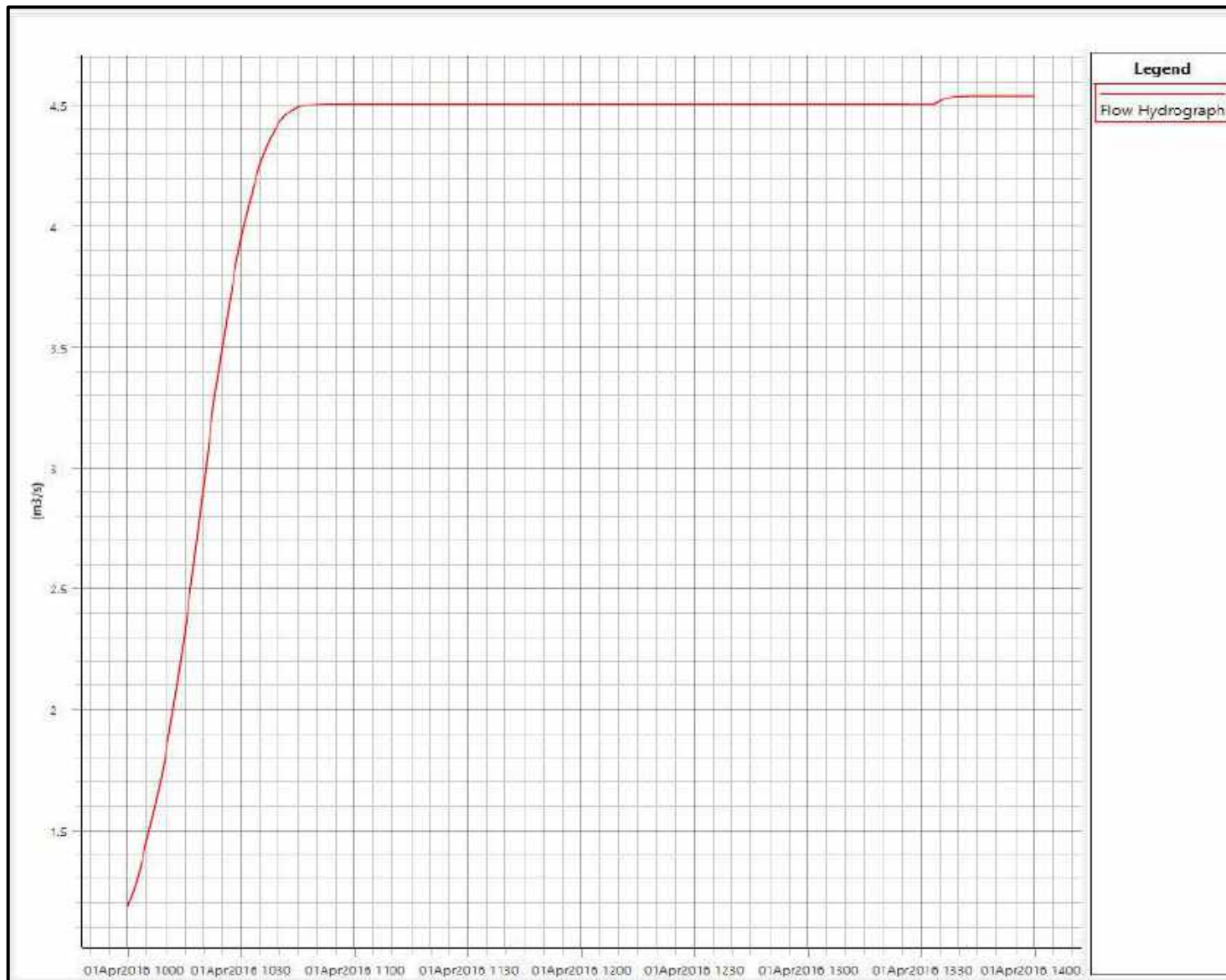
Figure E4 : Inflow Hydrograph at Boundary TGC01.24T
