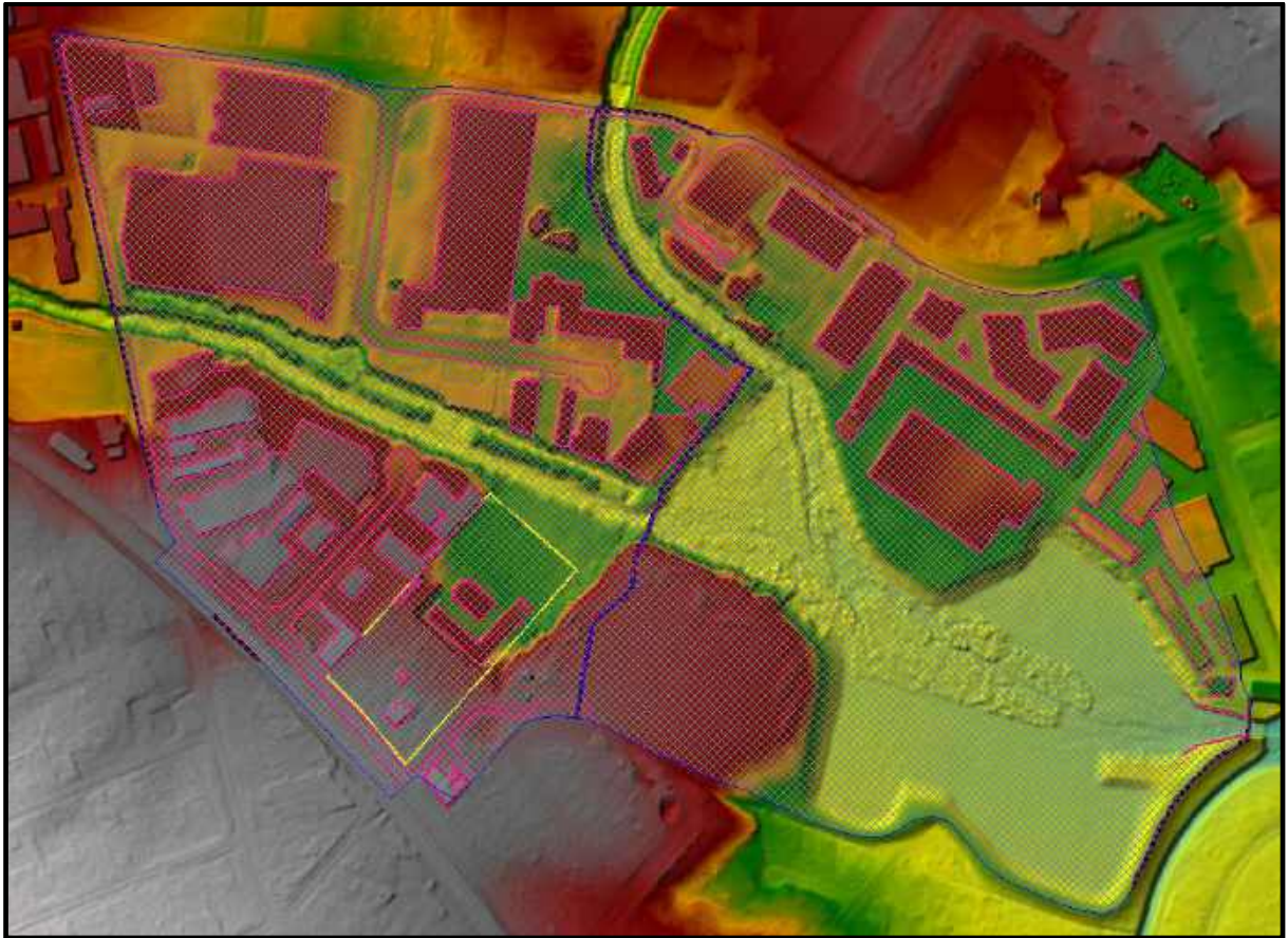
Figure 6 : Existing Hec-Ras 2D Model Layout (from Geometric Data Viewer)
