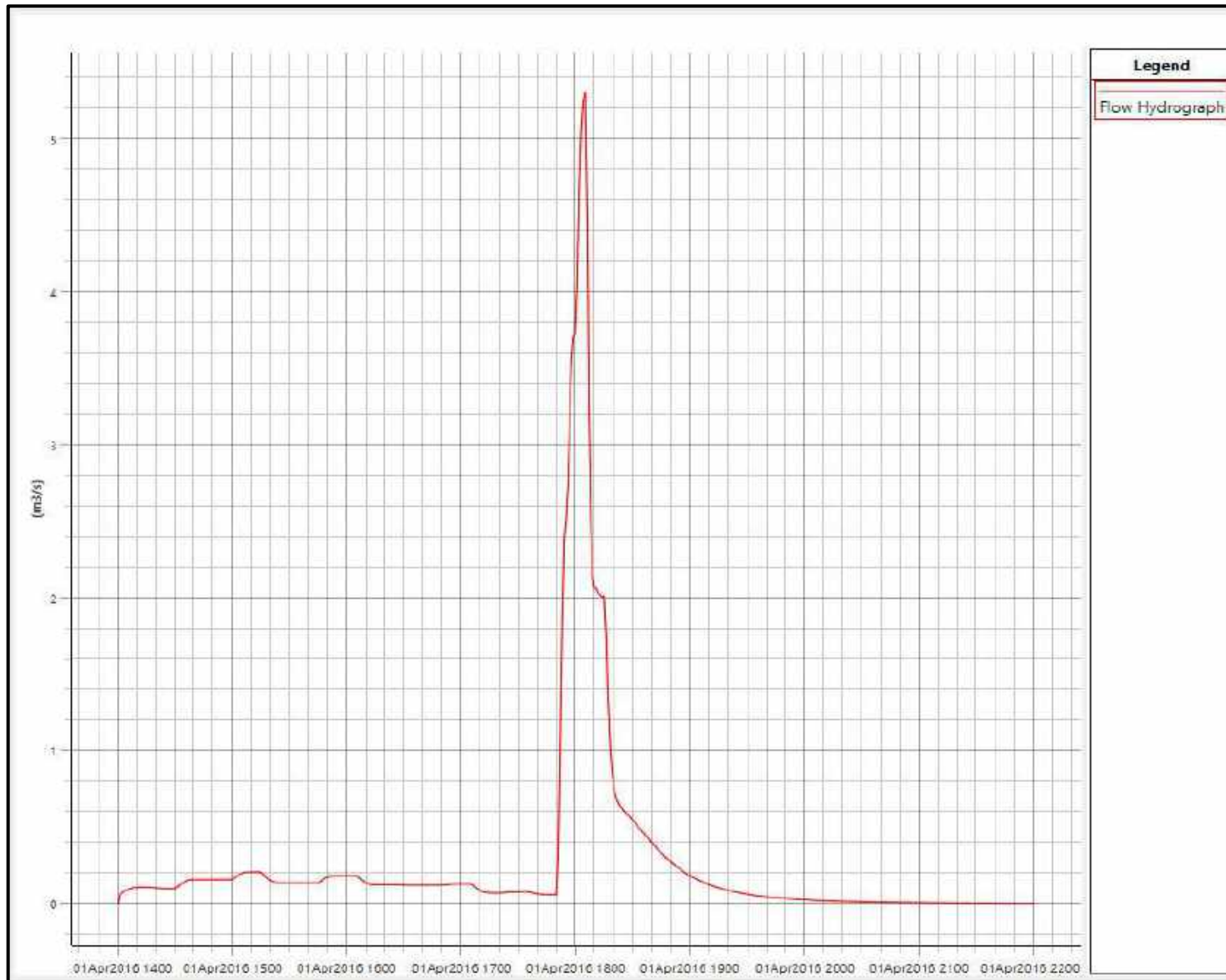
Figure E33 : Inflow Hydrograph at Boundary BTN31.00T
