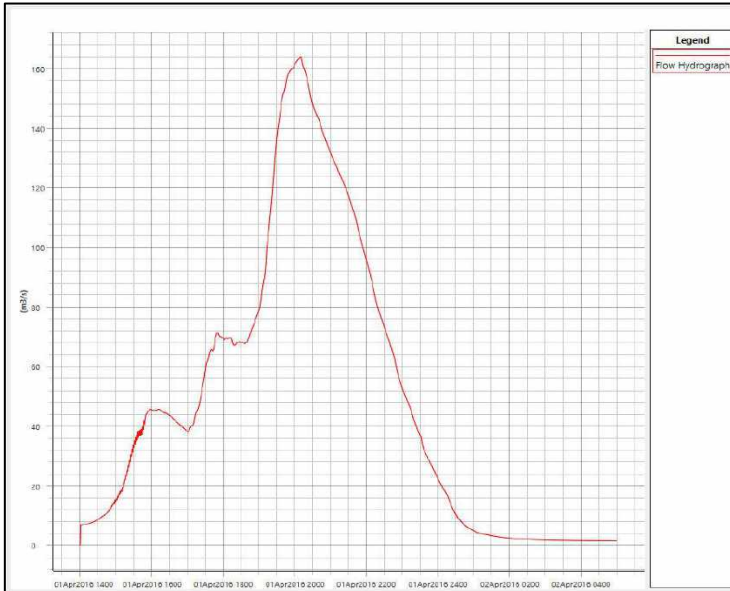
Figure E12 : Inflow Hydrograph at Boundary BTN01.38T
