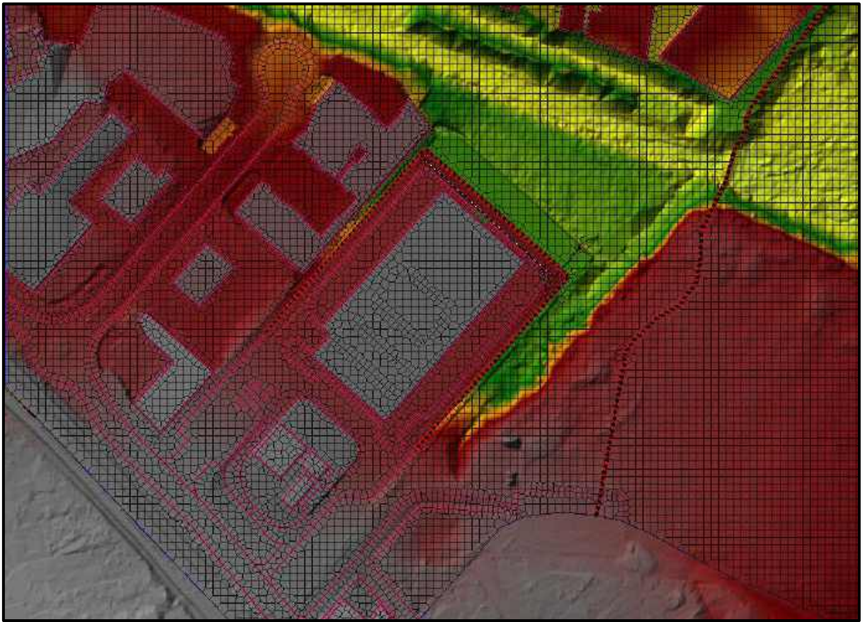
Figure 9 : HEC-RAS 6 model Terrain Grid, Design Scenario (from Geometric Data)
