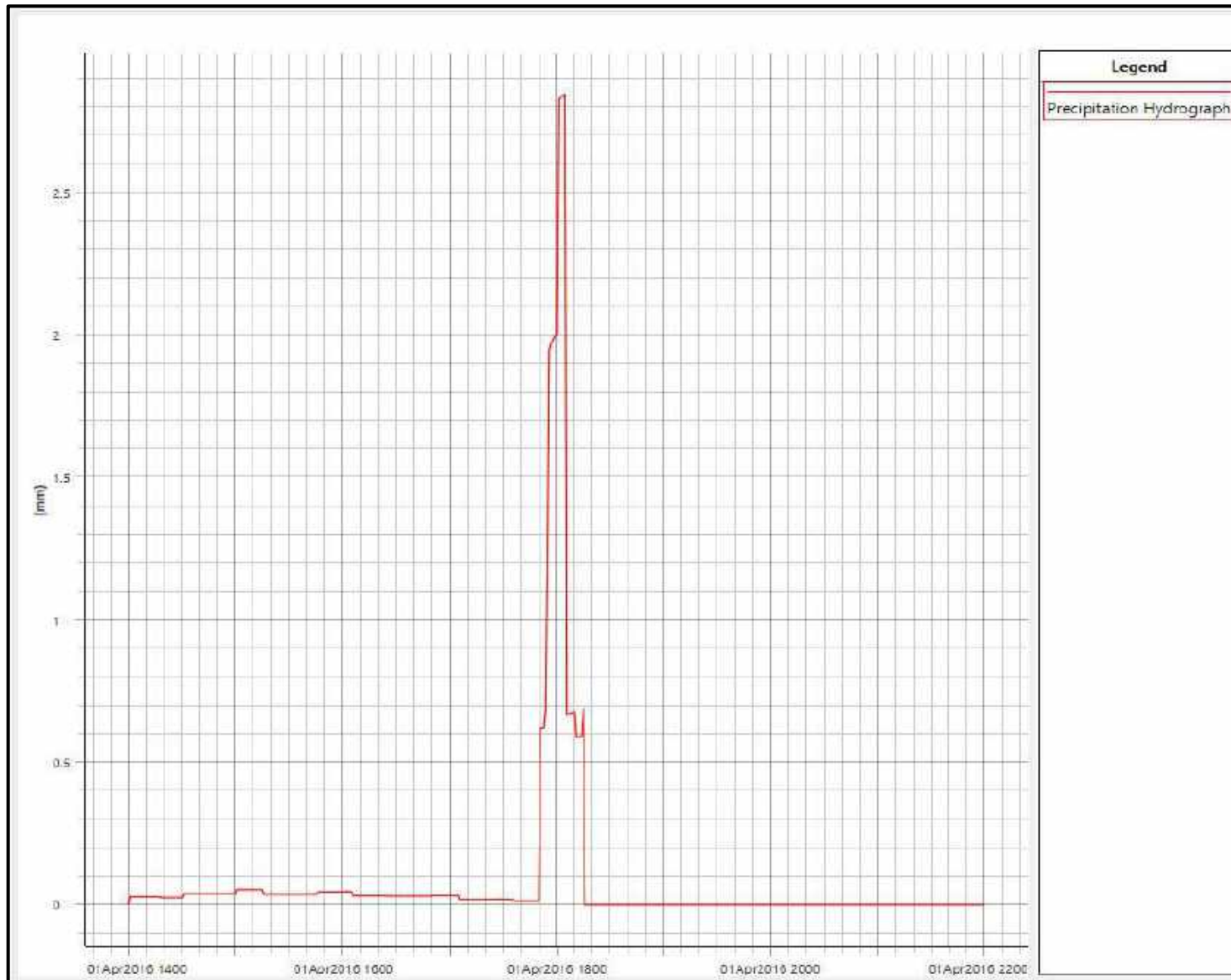
Figure E36 : Precipitation Excess for Flow Area McCoy_FA
