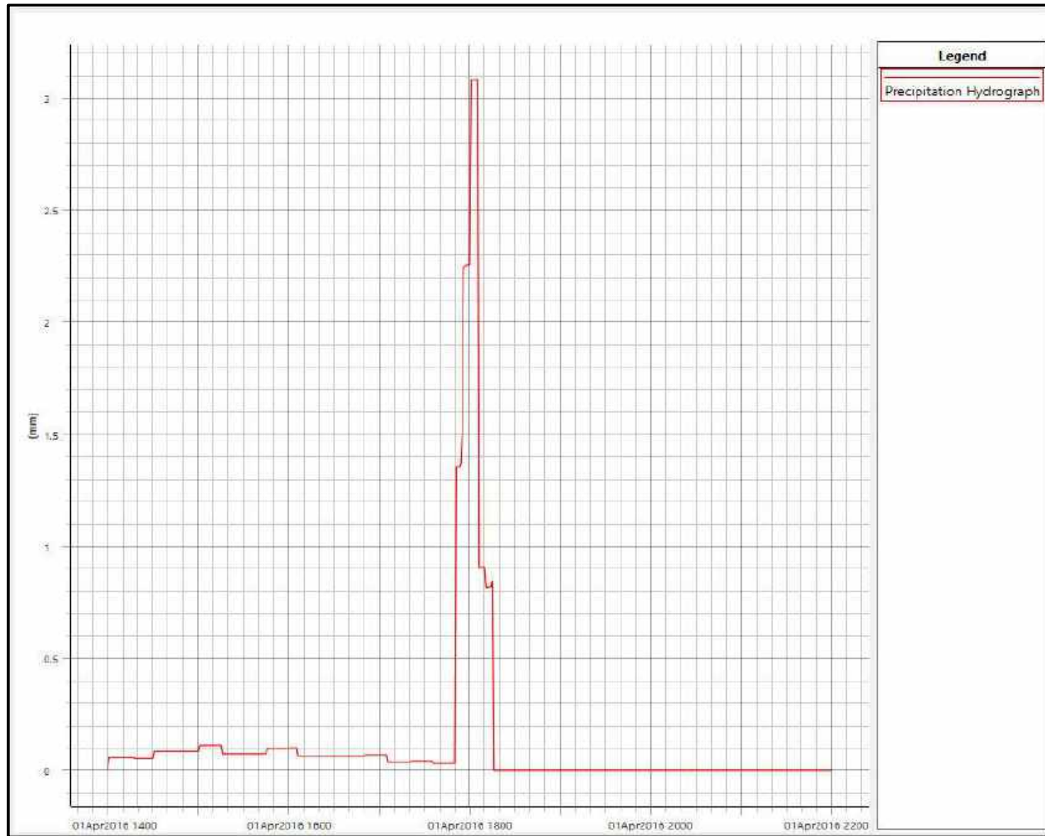
Figure E35 : Precipitation Excess for Flow Area StationRd_FA
