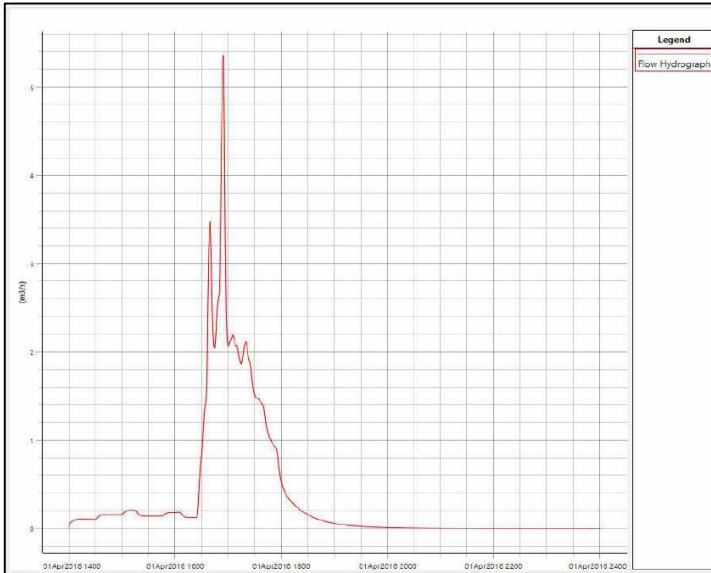
Figure E28 : Inflow Hydrograph at Boundary BTN31.00T
