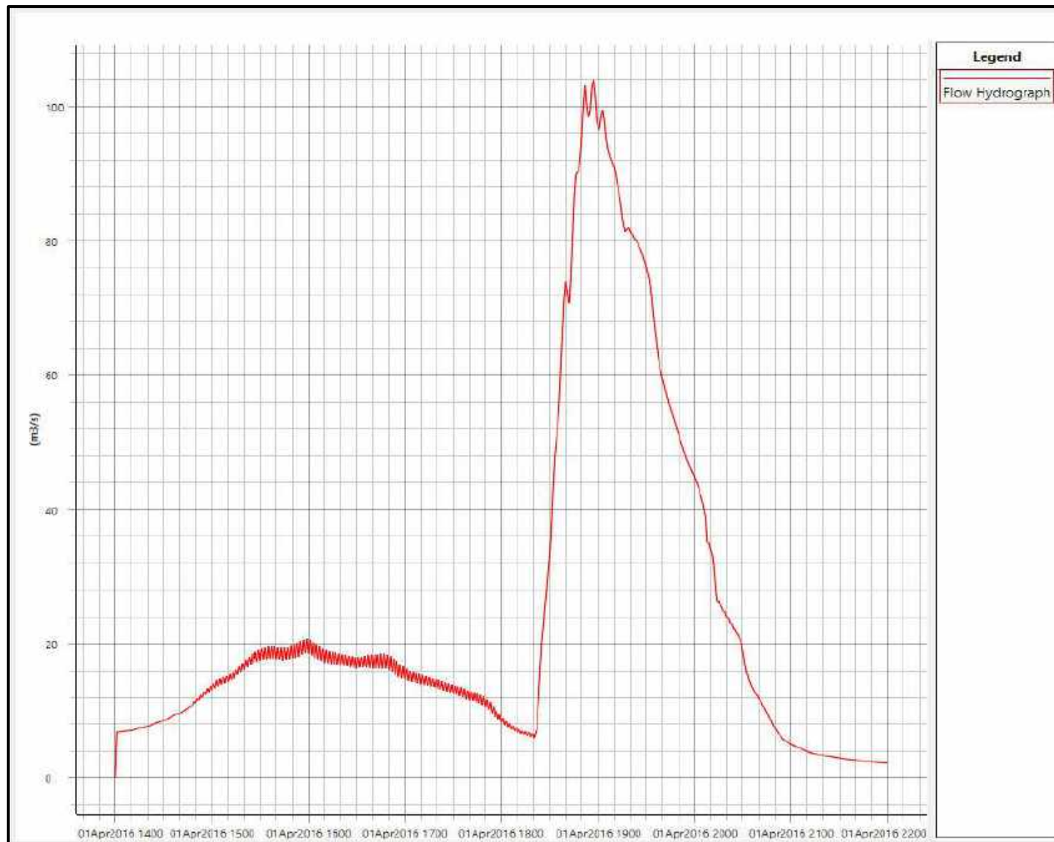
Figure E37 : Inflow Hydrograph at Boundary BTN01.38T
