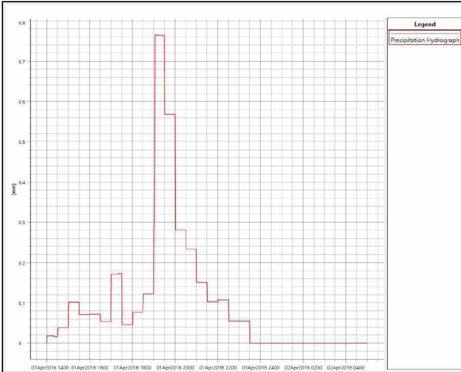
Figure E21 : Precipitation Excess for Flow Area McCoy_FA
