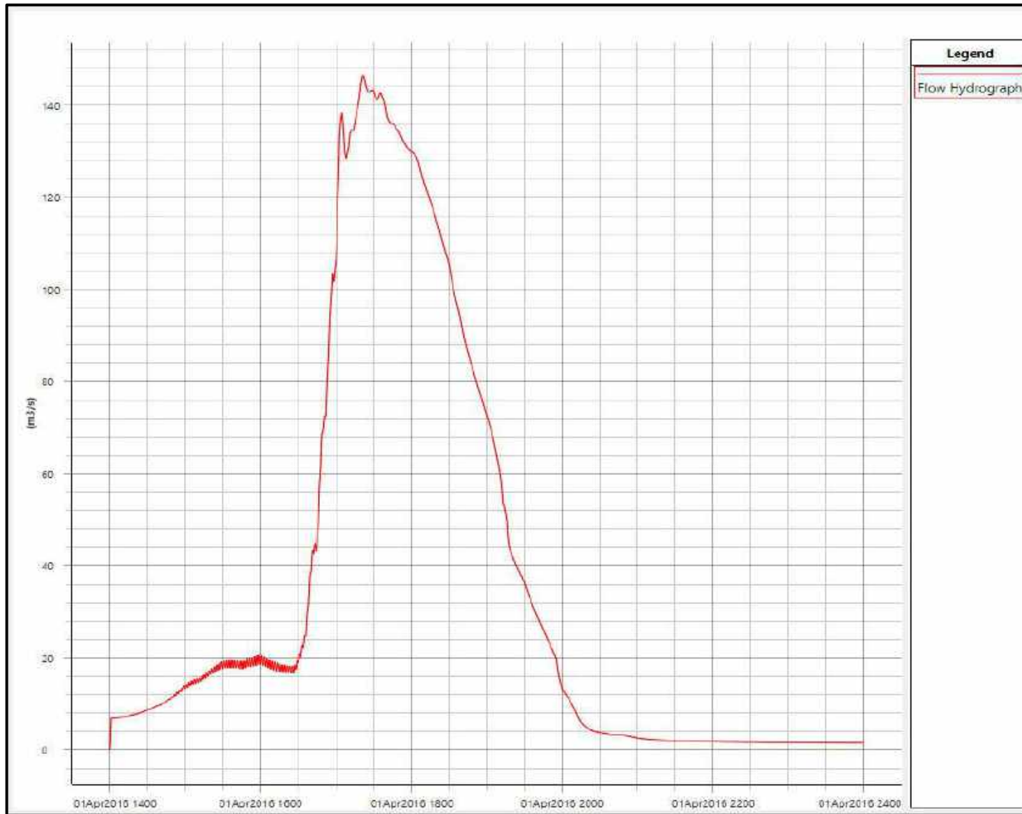
Figure E27 : Inflow Hydrograph at Boundary BTN01.38T
