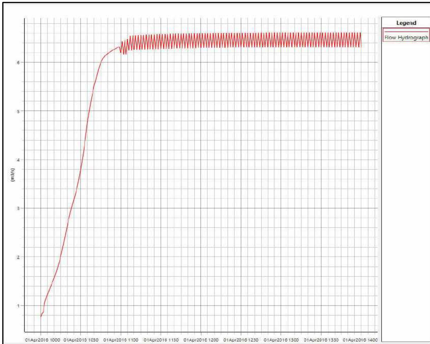
Figure E2 : Inflow Hydrograph at Boundary BTN01.38T
