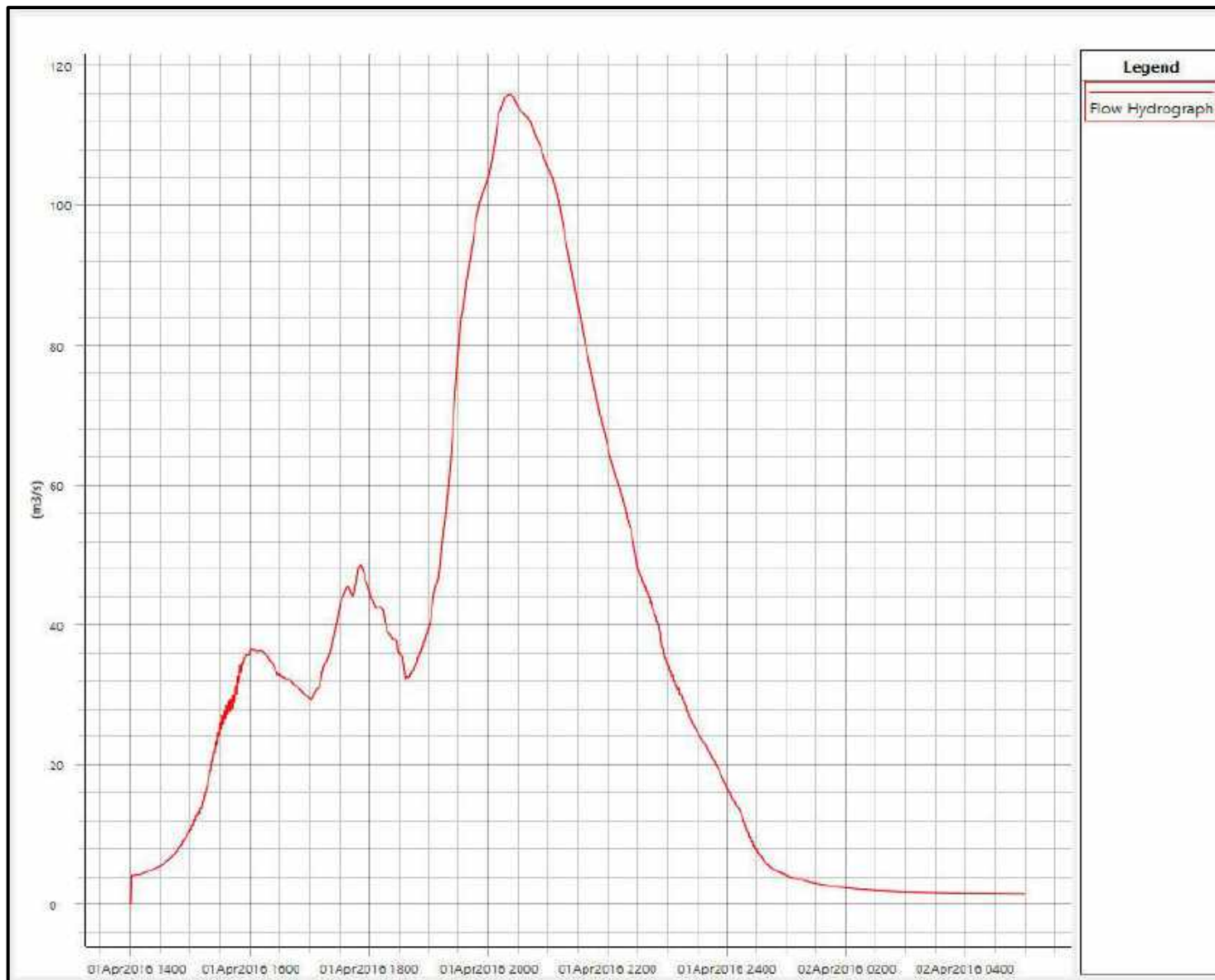
Figure E17 : Inflow Hydrograph at Boundary BTN01.38T
