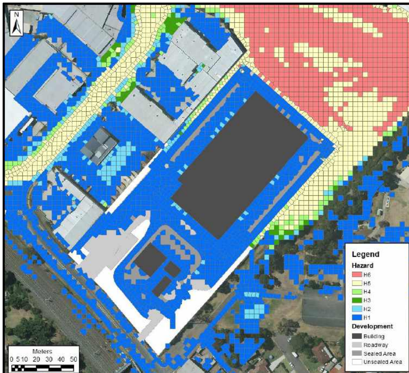
Figure G11: Design 60 min PMF AEP Hydraulic Hazard for the Site.
