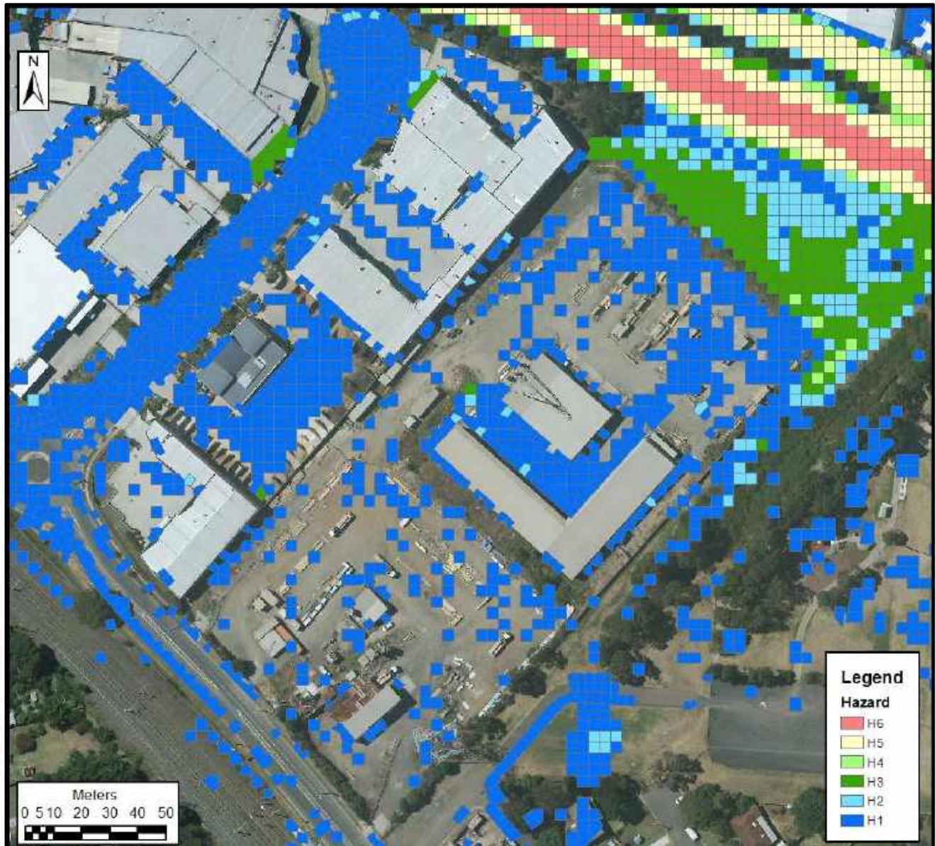
Figure G2: Existing 9 hour 5% AEP Hydraulic Hazard for the Site.
