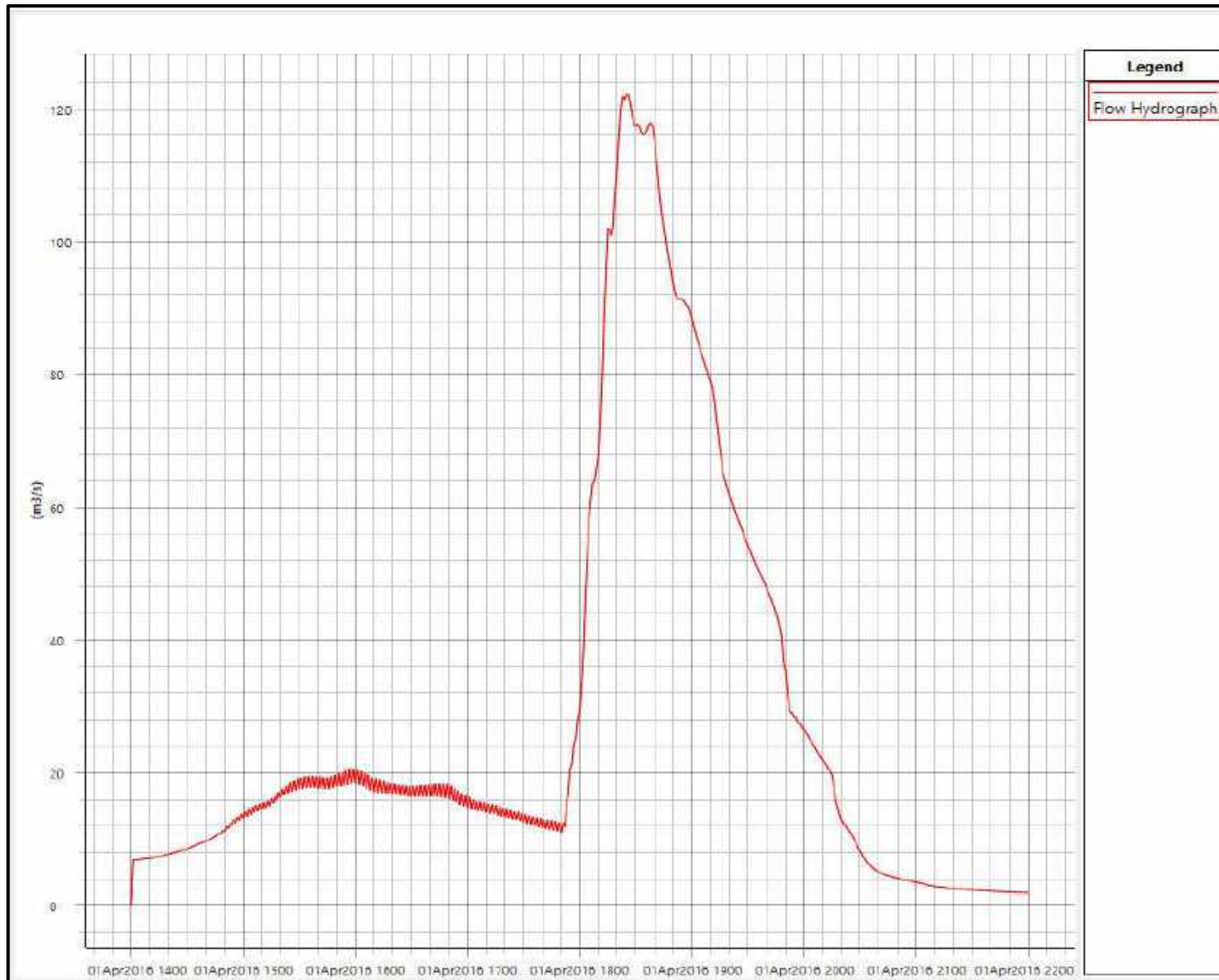
Figure E32 : Inflow Hydrograph at Boundary BTN01.38T
