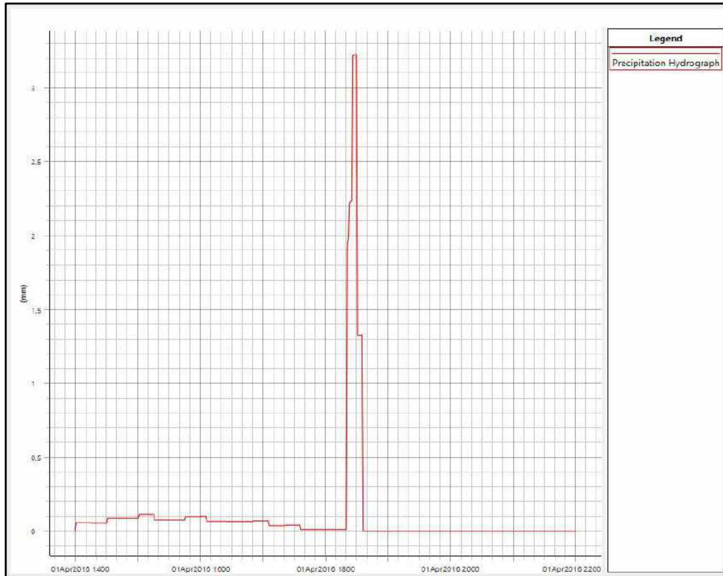
Figure E40 : Precipitation Excess for Flow Area StationRd_FA
