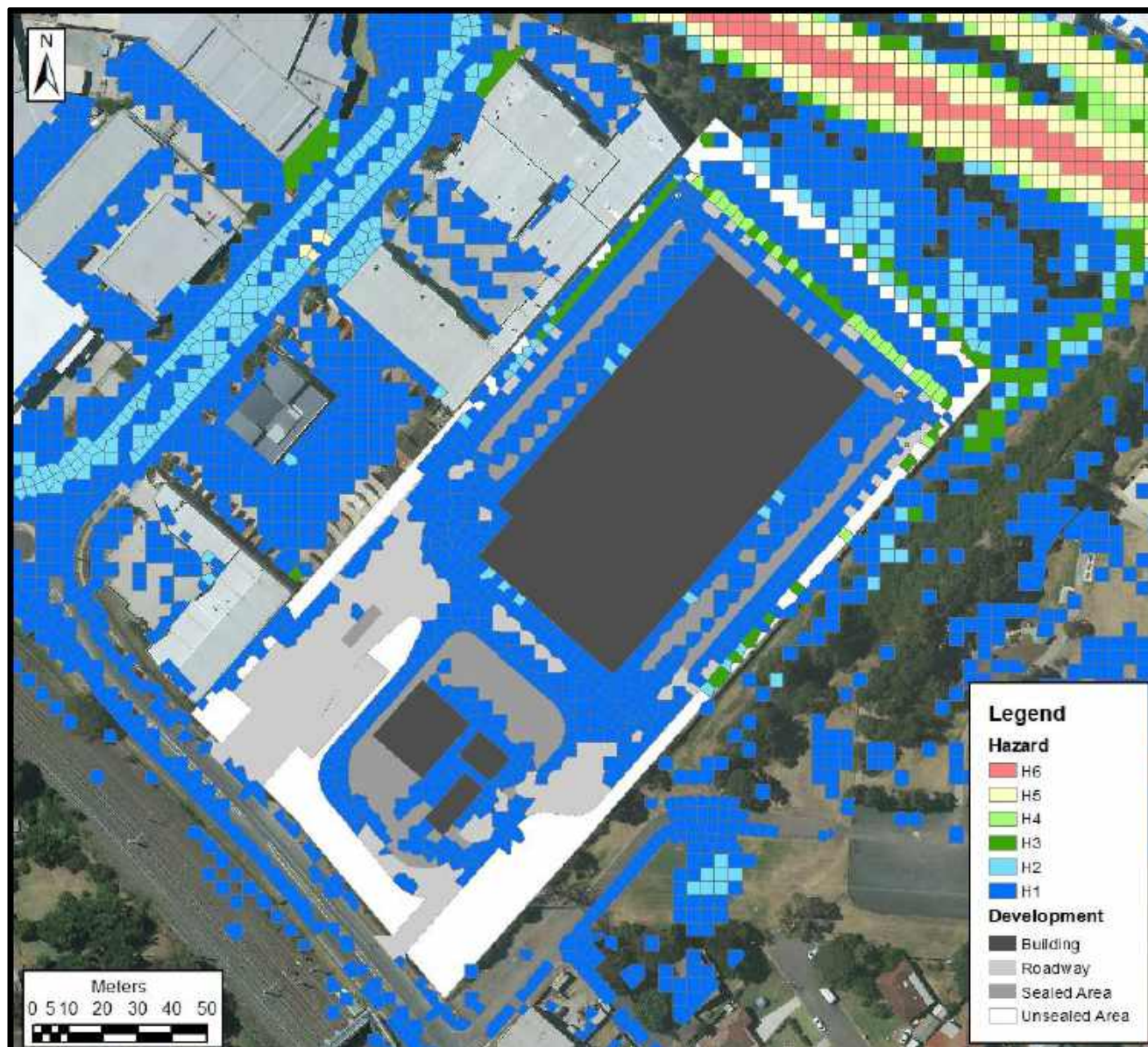
Figure G10: Design 15 min 1% AEP Hydraulic Hazard for the Site.
