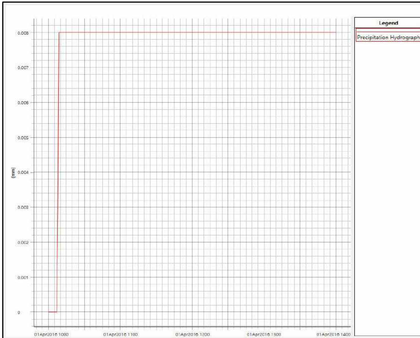
Figure E11 : Precipitation Excess for Flow Area McCoy_FA
