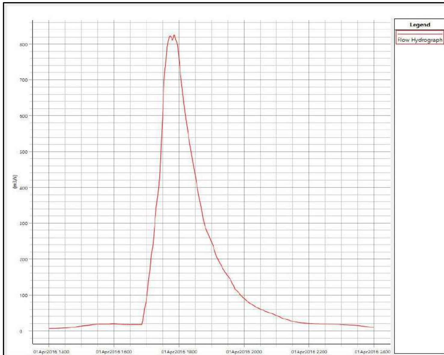
Figure E22 : Inflow Hydrograph at Boundary BTN01.38T
