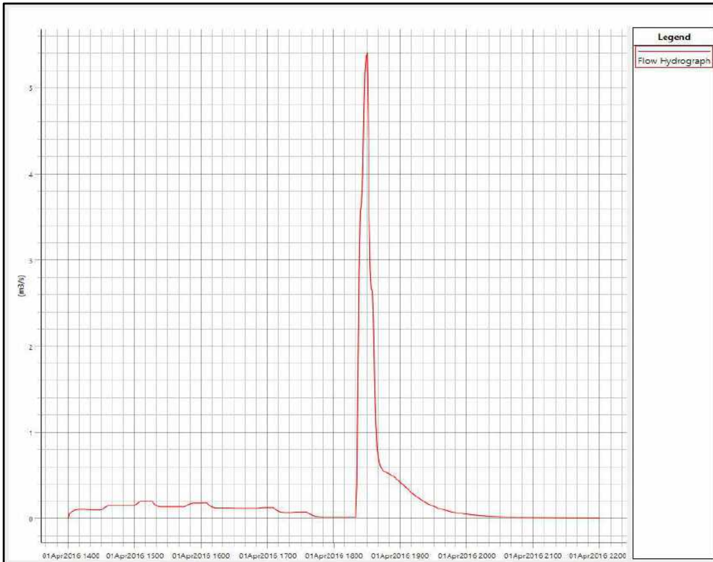
Figure E38 : Inflow Hydrograph at Boundary BTN31.00T
