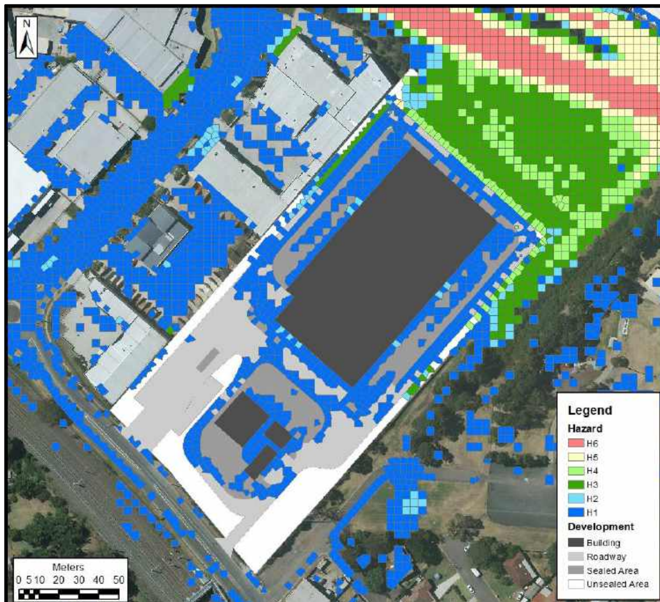
Figure G6: Design 9 hour 1% AEP Hydraulic Hazard for the Site.
