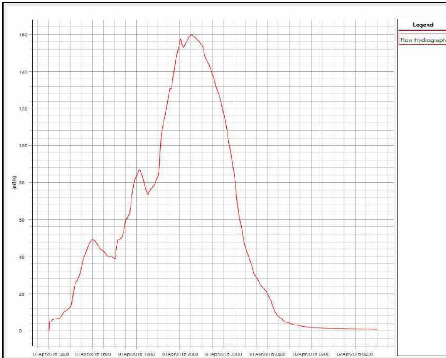
Figure E14 : Inflow Hydrograph at Boundary TGC01.24T
