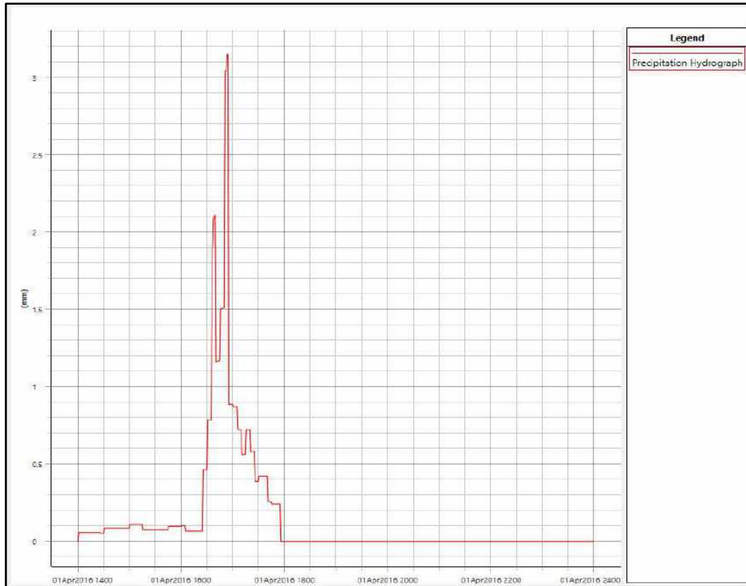
Figure E30 : Precipitation Excess for Flow Area StationRd_FA
