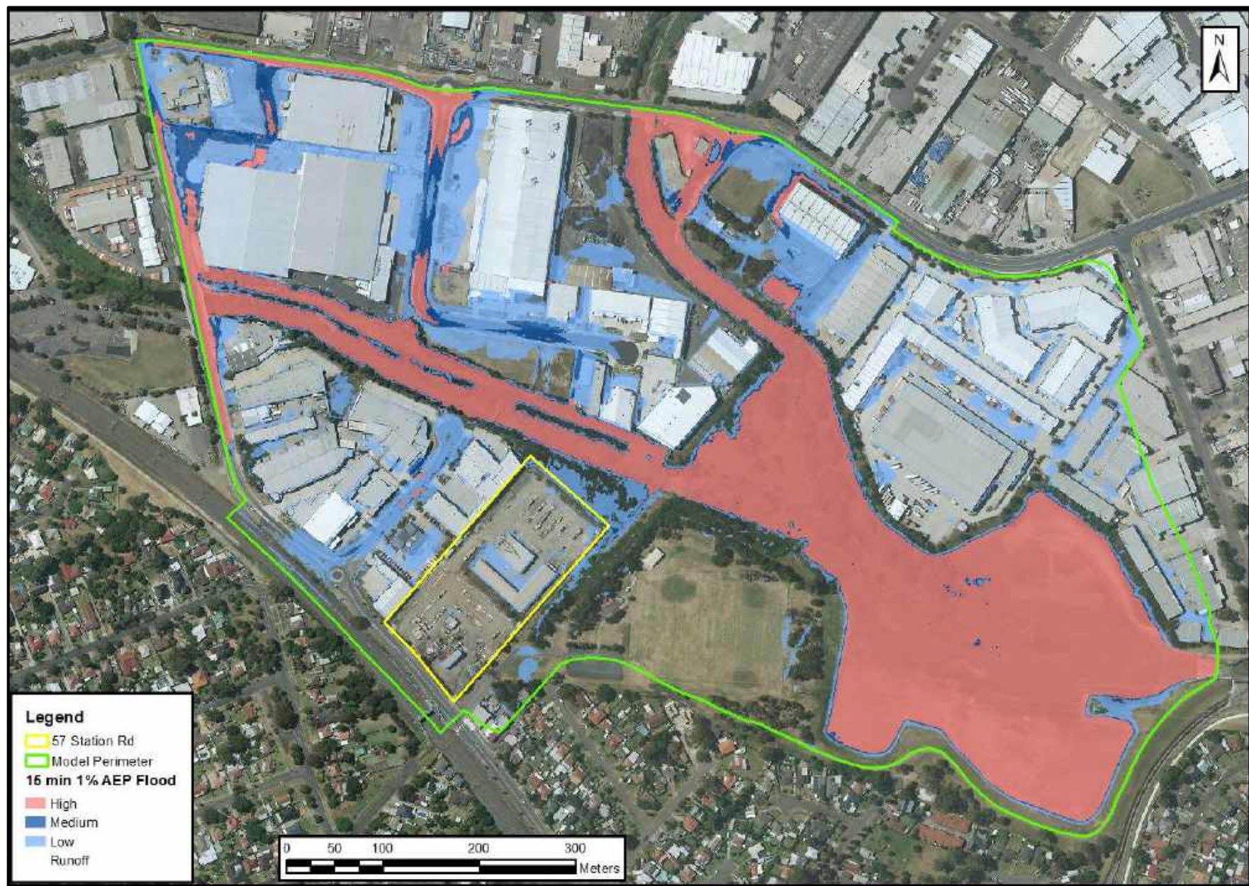
Figure F5: Existing 15 min 1% AEP Flood Extent
