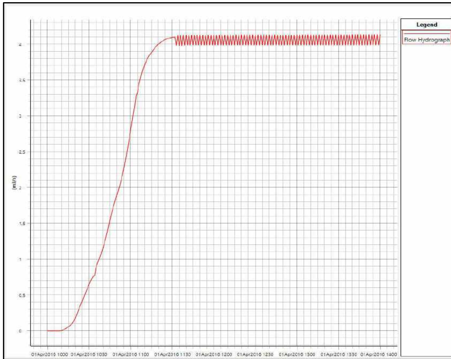
Figure E7 : Inflow Hydrograph at Boundary BTN01.38T
