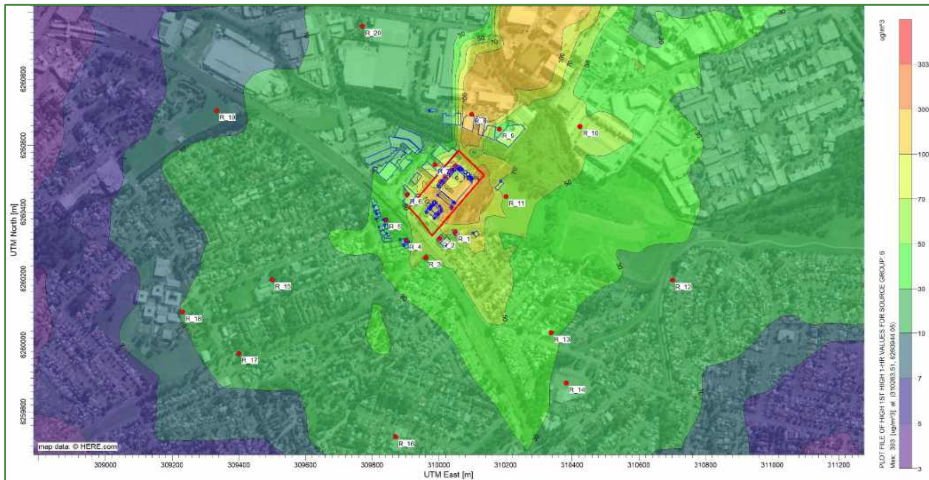
Figure 7-8: Isopleth for CO 1 hour – 100th Percentile (without background)
