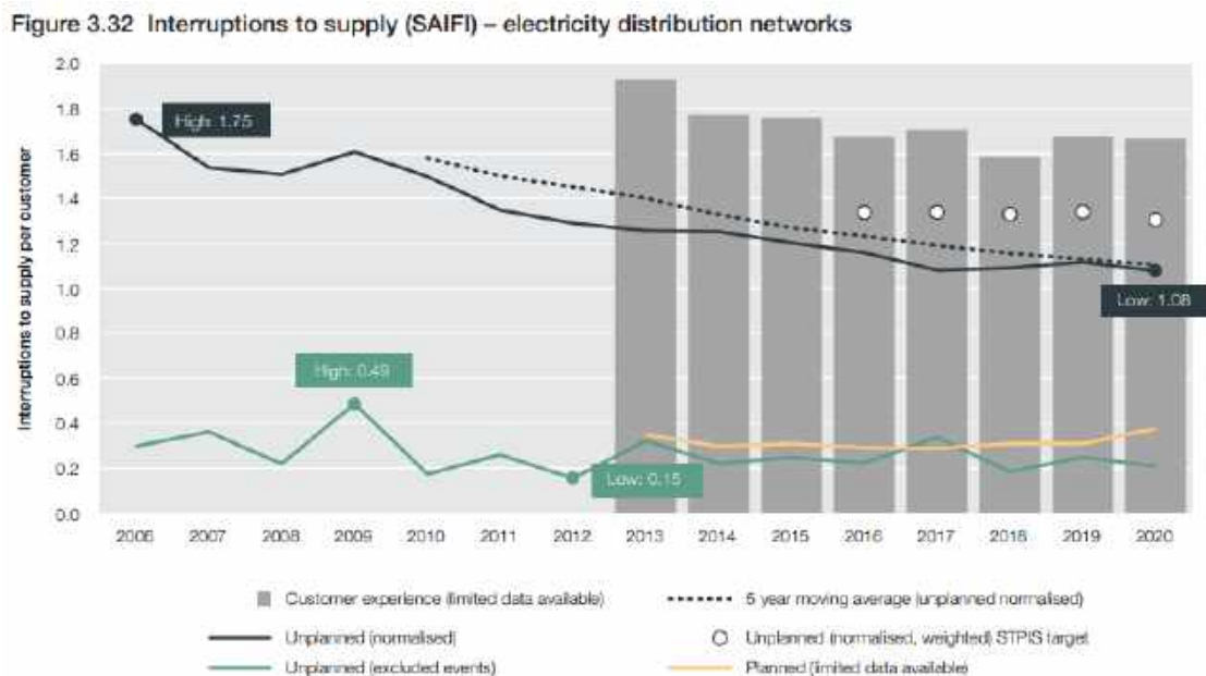
Figure 7-1: Reproduced Figure 3.32 from 'State of the energy market 2021' report published by Australian Energy Regulator (AER) - system average interruption frequency index (SAIFI).
