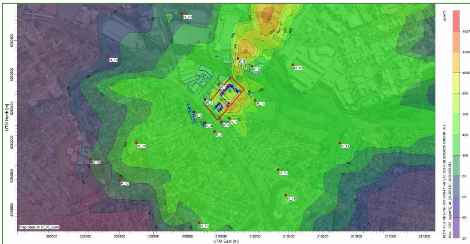
Figure 7-7: Isopleth for NO x – 100th Percentile (without background)
