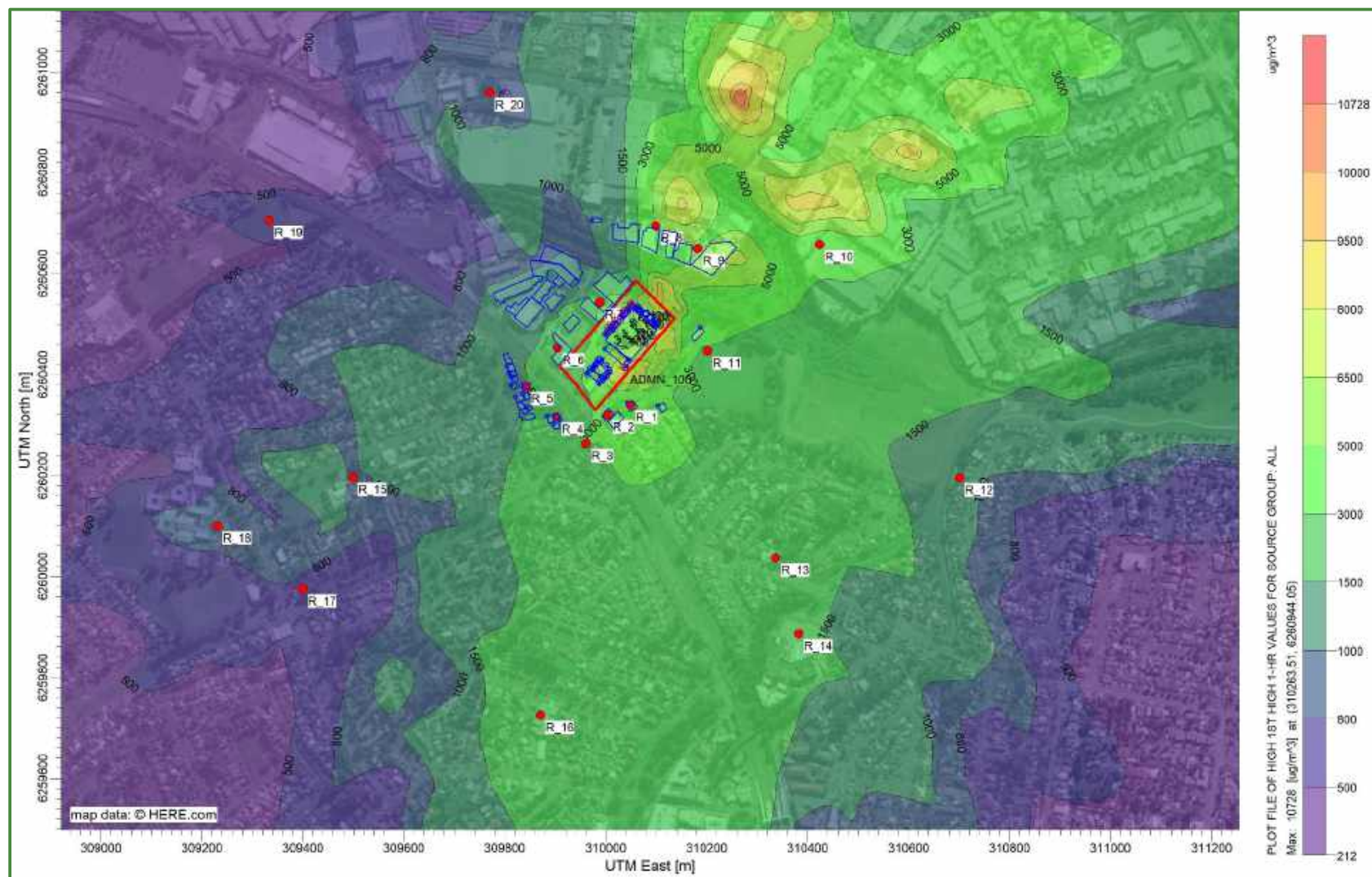
Figure 7-12: Isopleth for NOx – 100th Percentile (without background)
