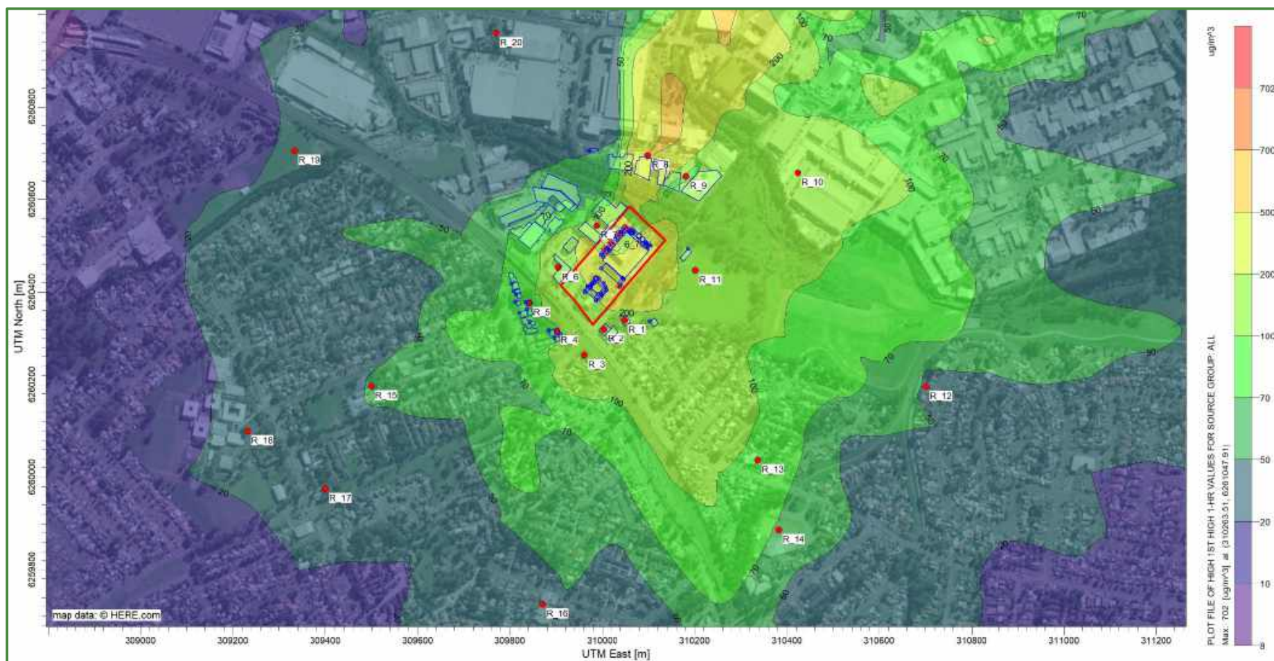
Figure 7-6: Isopleth for NO x – 100 th Percentile (without background)
