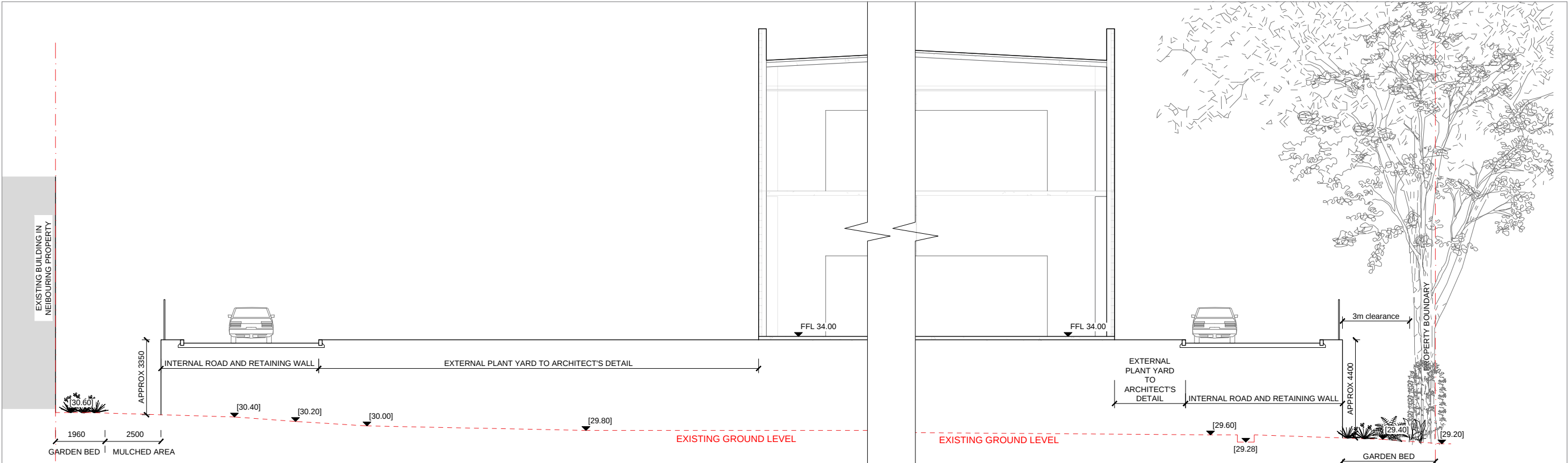
SECTION 1-1 PART A
