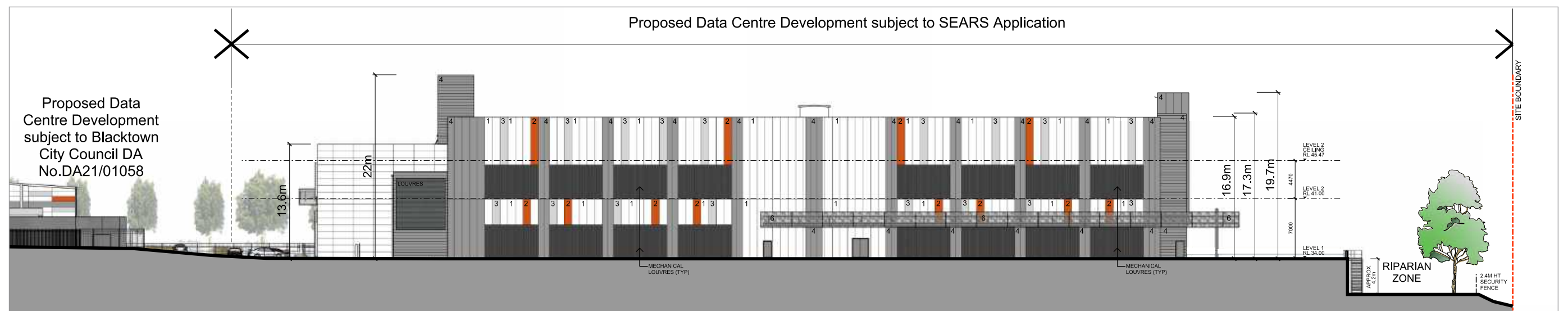
SOUTH-EAST ELEVATION
