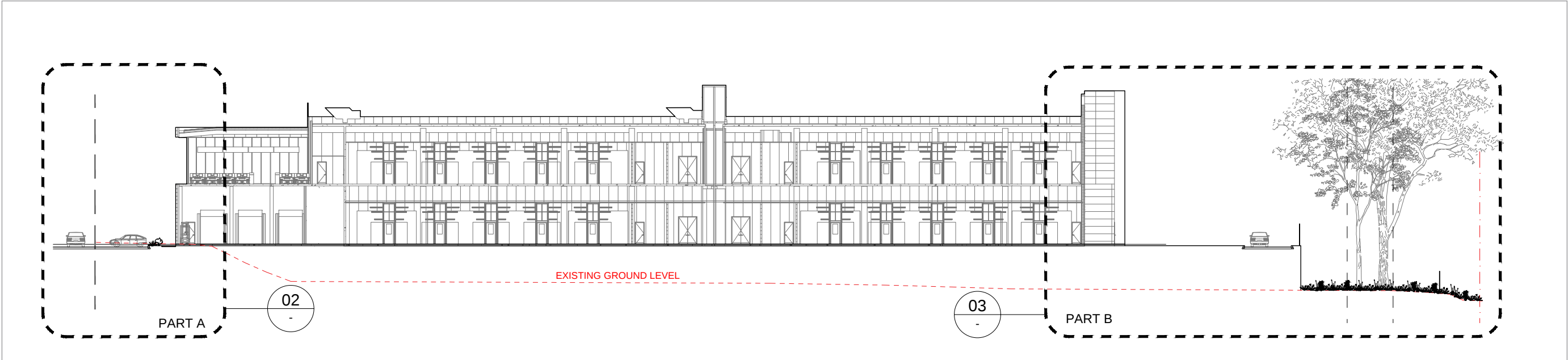
SECTION 2-2
