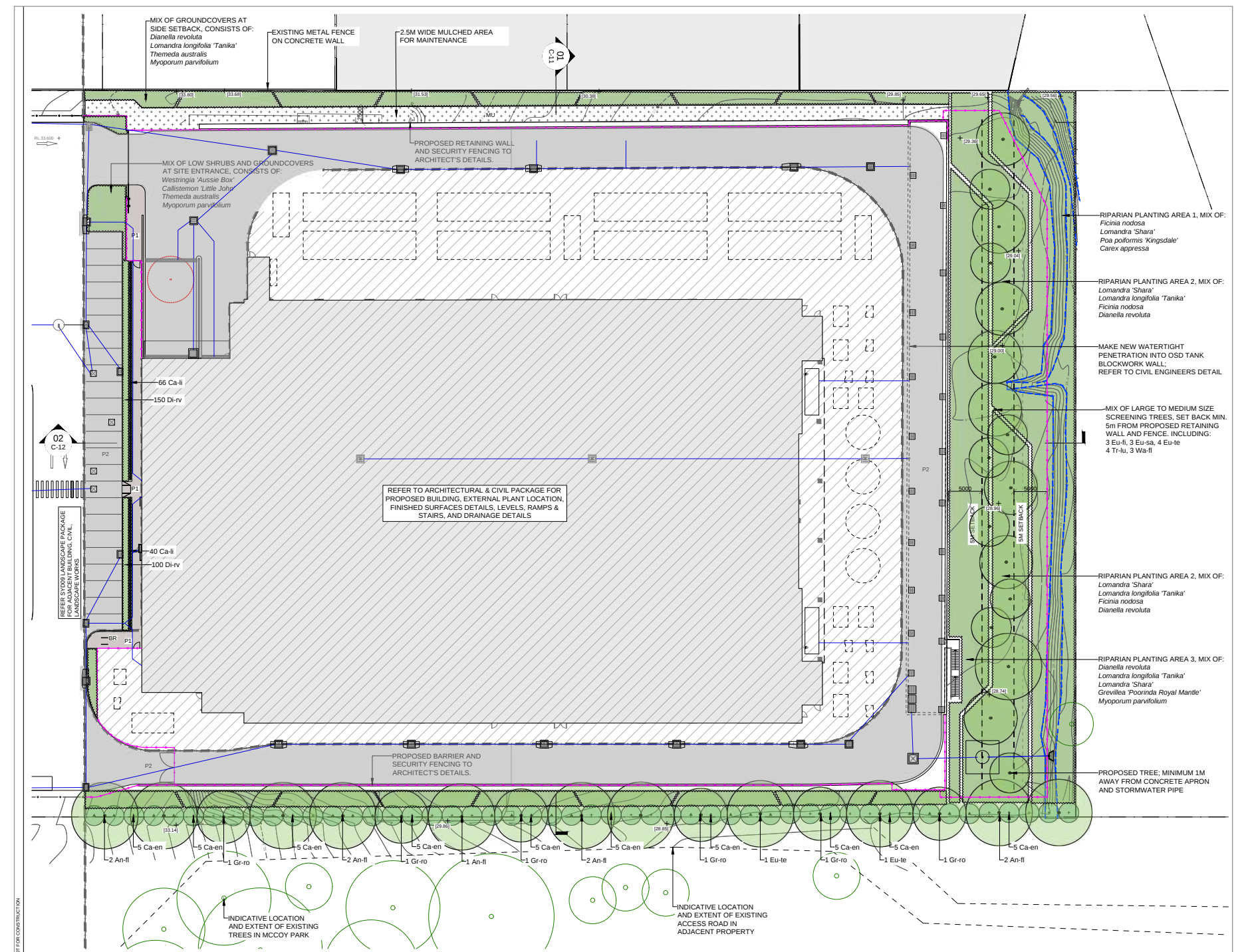
LANDSCAPE PLAN
