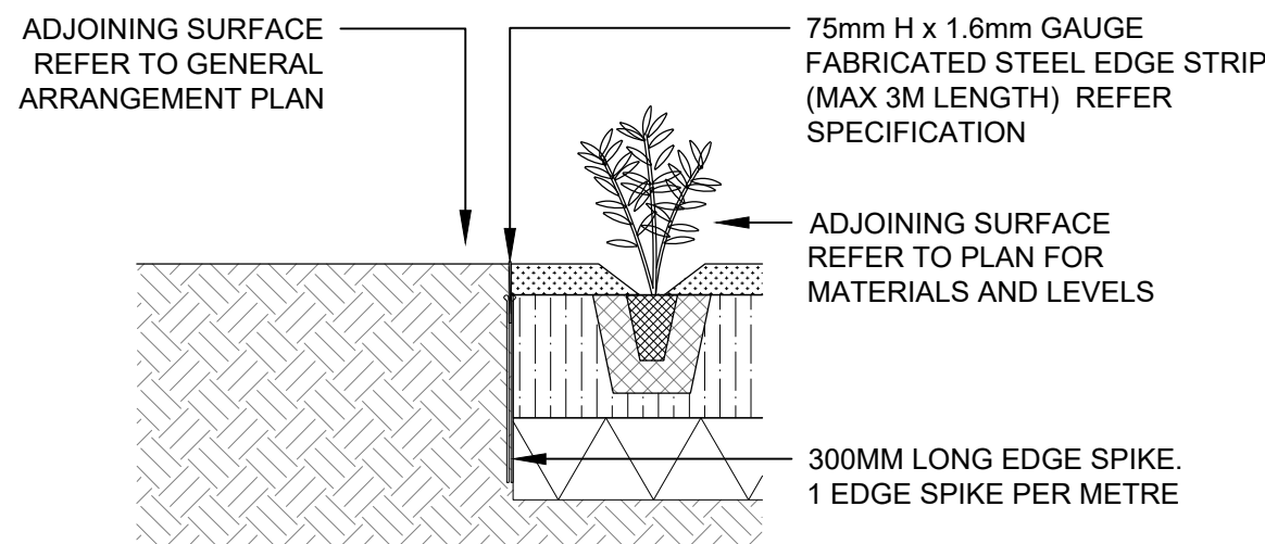
03 STEEL GARDEN EDGE TYPICAL DETAIL 1:20
