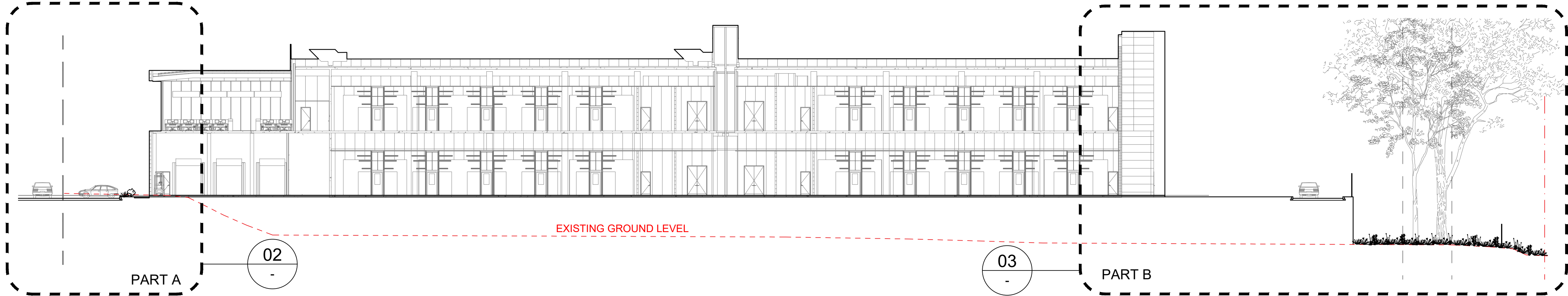
01 SECTION 02 1:250 @ A1
